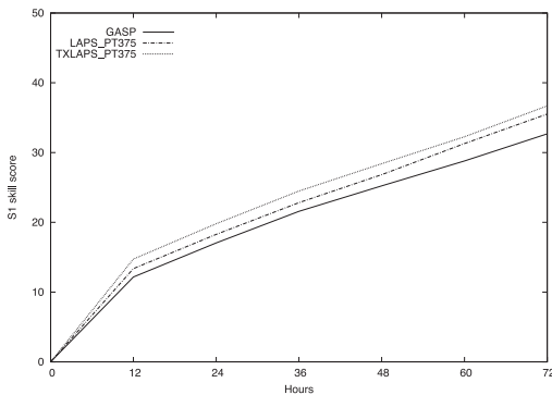
Fig. 1(b) 500 hPa geopotential height S1 skill score comparison, for different forecast periods, between GASP, LAPS_PT375 and TXLAPS_PT375 (October to December 2006).
