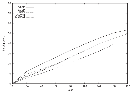
Fig. 2(b) 500 hPa geopotential height S1 skill score comparison, for different forecast periods, between GASP, ECSP, UKGC, USAVN and JMAGSM (October to December 2006).
