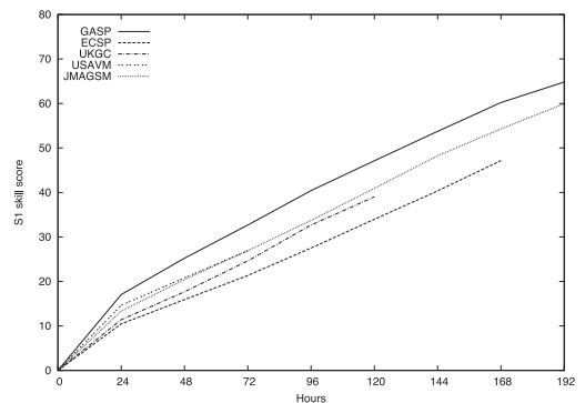
Fig. 2(b) 500 hPa geopotential height S1 skill score comparison, for different forecast periods, between GASP, ECSP, UKGC, USAVN and JMAGSM (October to December 2006).
