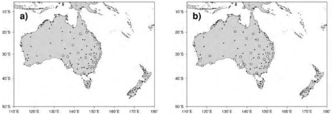
Fig. 6 Locations where a significant change (open circles) in the mean and (1 or 2) extremes over the period 1961 to 2005 was observed: (a) Tmax, (b) Tmin. All other station locations are also shown (solid dots).
