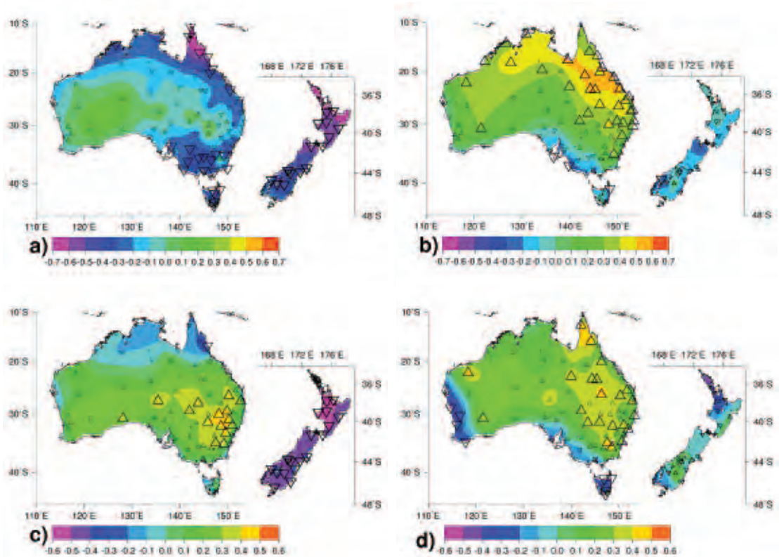
Fig. 12 Correlations between (a) detrended JJA NINO3.4 index (same year) and detrended Tmin, (b) detrended DJF NINO3.4 (same year) and detrended Tmax and (d) detrended DJF NINO3.4 (same year) and WN. Statistical significance (at the 5% level) and the sign of the correlation at the individual stations is indicated by triangles – bold large triangles representing significant correlations, positive (negative) correlations represented by up (down) facing triangles.
