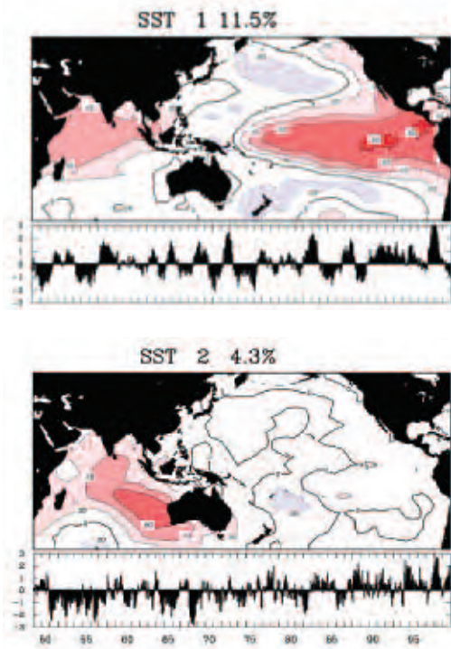
Fig. 3 First two VARIMAX rotated principal components of near-global sea-surface temperature patterns together with the time series of their amplitudes, 1949 to 1999 (Drosowsky and Chambers 2001).
