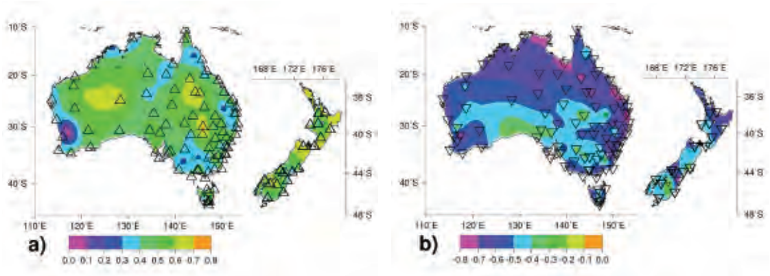
Fig. 10 Correlations with Tmin (a) warm nights and (b) cold nights, 1961-2005. Statistical significance (at the 5% level) and the sign of the correlation at the individual stations is indicated by triangles – bold large triangles representing significant correlations, positive (negative) correlations represented by up (down) facing triangles.
