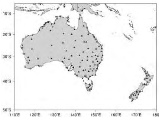
Fig. 2 Urban status of the stations. Highly urban sites (population was greater than 300 000 with more than 300 people per km 2 in 2001) (circles), urban sites (either the population was greater than 300 000 or more than 300 people per km 2 , but not both) (squares) and rural sites (less than 300 000 people and density less than 300 per km 2 ) (triangles).
