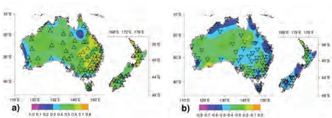
Fig. 9 Correlations with Tmax (a) hot days and (b) cool days, 1961-2005. Statistical significance (at the five per cent level) and the sign of the correlation at the individual stations is indicated by triangles – bold large triangles representing significant correlations, positive (negative) correlations represented by up (down) facing triangles.
