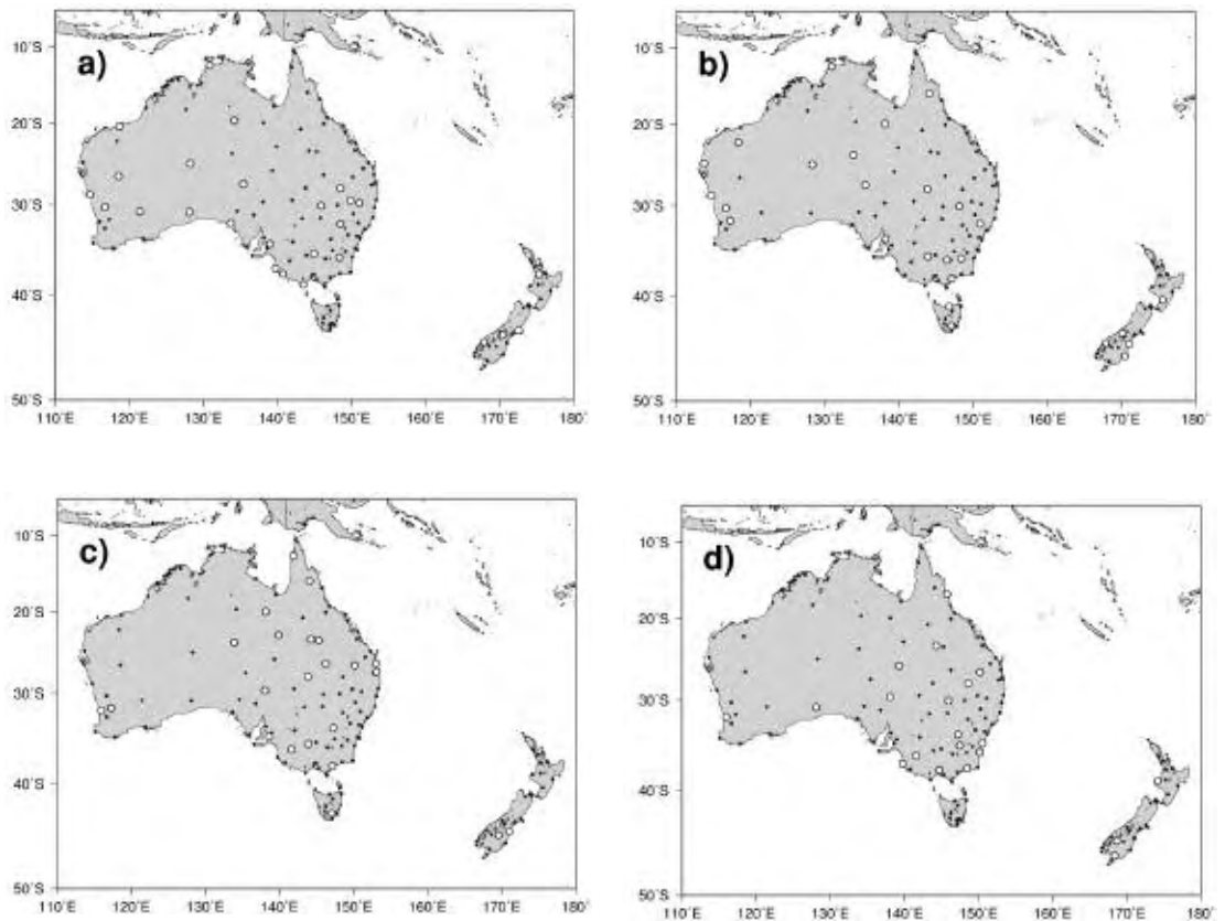
Fig. 7 Locations where no distributional change was detected (open circles) over the period 1961-2005: (a) Tmax (b) Tmin; or there was a change in mean only: (c) Tmax, (d) Tmin. All other station locations are also shown (solid dots).
