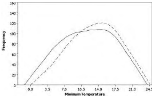
Fig. 13 Daily minimum temperature distribution at Port Macquarie; 1931 to 1941 (black line) compared to 1991 to 2005 (dashed line) (Lowess smoothed probability density functions with 0.2 degrees of smoothing).
