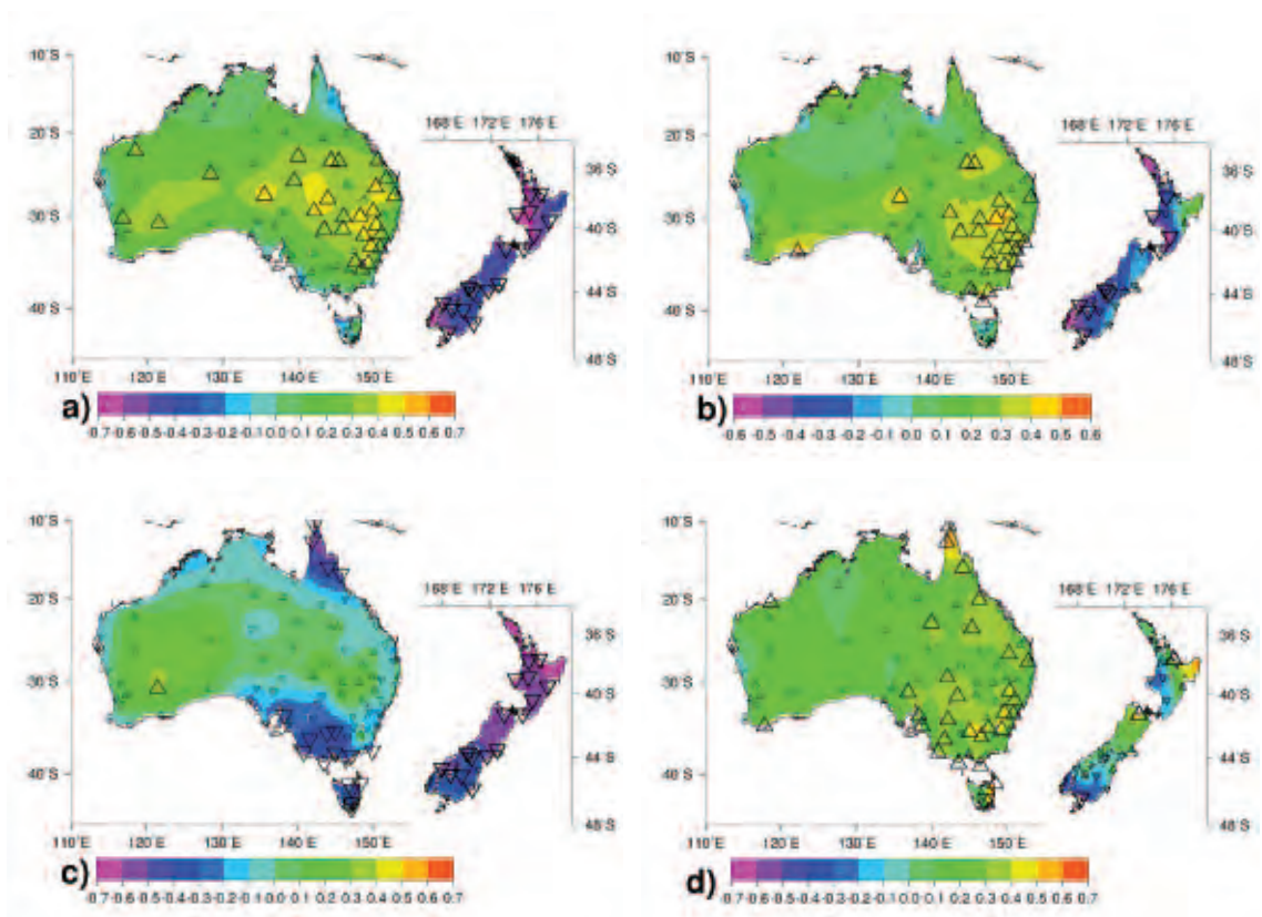
Fig. 11 Detrended annual NINO3.4 index (same year), correlated with detrended (a) Tmax, (b) HD, (c) Tmin and (d) DTR. Statistical significance (at the 5% level) and the sign of the correlation at the individual stations is indicated by triangles – bold large triangles representing significant correlations, positive (negative) correlations represented by up (down) facing triangles.
