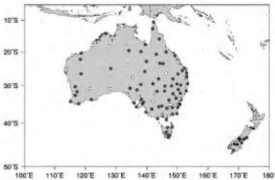
Fig. 1 Station location and data duration: 17 stations with 1931-2005 data (black stars), 36 stations with 1946-2005 data (white squares), and 65 stations with 1961-2005 data (grey circles). Note that, for example, all 118 stations with data present over the 1961-2005 period are used in the 1961-2005 analysis, and that similarly, 53 stations with data present over the 1946-2005 period are used in the 1946-2005 analysis.
