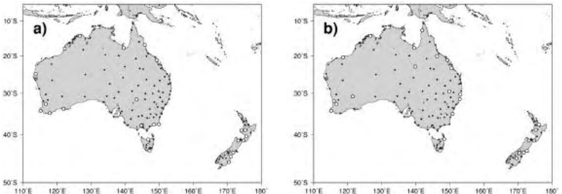
Fig. 8 Locations where a change in the standard deviation was detected (open circles) over the period 1961-2005: (a) Tmax, (b) Tmin. All other station locations are also shown (solid dots).
