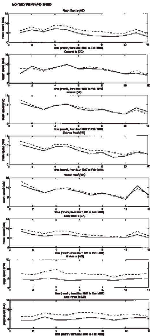
Fig. 2 The monthly mean time series of the surface winds from March 1997 to February 1998. The solid line indicates AWS winds and the dashed line the LAPS forecast.
