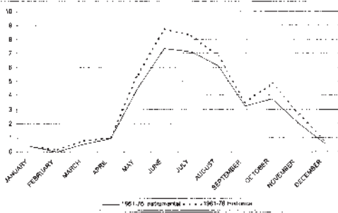
Fig. 3 Comparison between the instrumental (at Puente del Inca) and historical series of average numbers of snow days between 1961 and 1976.
