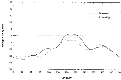
Fig. 12 Mean southern hemisphere blocking index for summer 2002/03 (solid line). The dashed line shows the corresponding long-term average. The horizontal axis shows degrees east of the Greenwich meridian.
