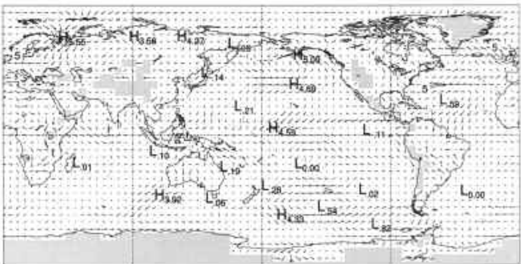
Fig. 13 Summer 2002/03 850 hPa vector wind anomalies with contours of vector magnitude overlaid. The contour interval is 5 \text{ m s}^{-1} , with values above 5 \text{ m s}^{-1} stippled.
