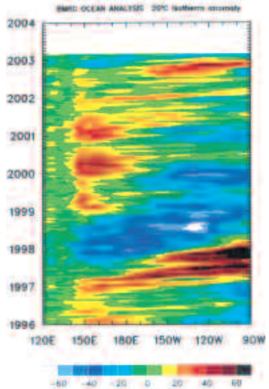
Fig. 4 Time-longitude section of the monthly anomalous depth of the 20°C isotherm at the equator from January 1996 to February 2003. The contour interval is 10 m.
