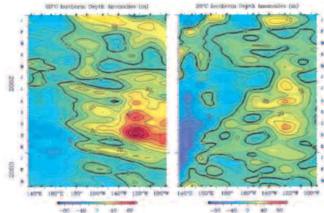
Fig. 5 Time-longitude sections of the monthly anomalous depth of the 20°C isotherm at (left) the equator and (right) 5°N from January 2002 to March 2003. The contour interval is 10 m.
