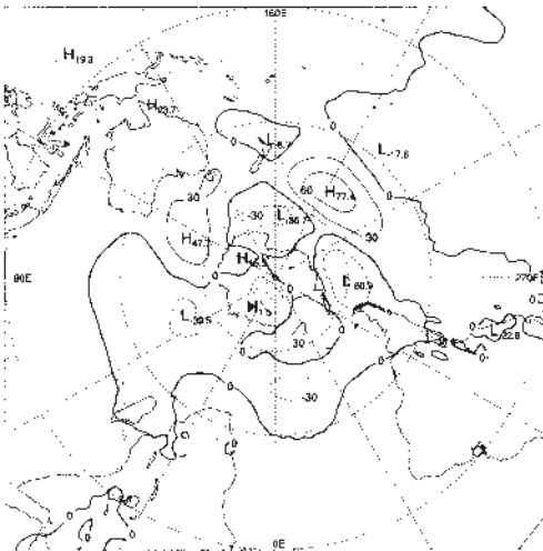
Fig. 10 Summer 2002/03 500 hPa geopotential height anomaly (gpm). The contour interval is 30 gpm, with values above 90 gpm and below -90 gpm stippled.
