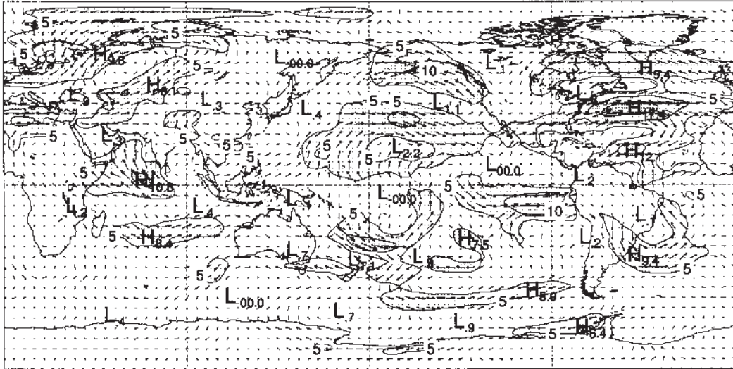
Fig. 14 Summer 2002/03 200 hPa vector wind anomalies with contours of vector magnitude overlaid. The contour interval is 5 \text{ m s}^{-1} , with values above 5 \text{ m s}^{-1} stippled.
