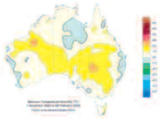
Fig. 18 Summer 2002/03 minimum temperature anomalies for Australia based on a 1961-1990 mean (°C).
