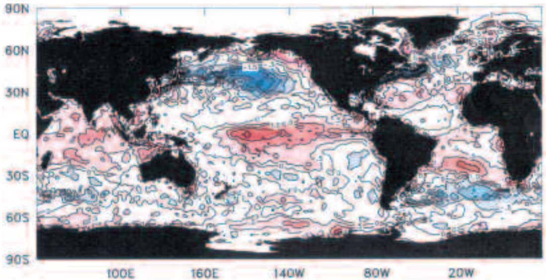
Fig. 3 Anomalies of sea-surface temperature for summer (December, January, February) 2002/03. The contour interval is 0.5°C.
