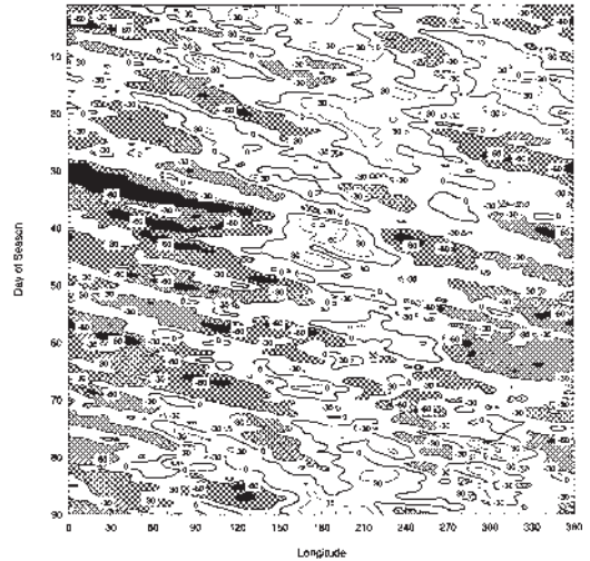
Fig. 11 Summer 2002/03 daily blocking index: time-longitude (Hovmoller) section. The horizontal axis measures degrees of longitude east of the Greenwich meridian. Day one is 1st December 2002.
