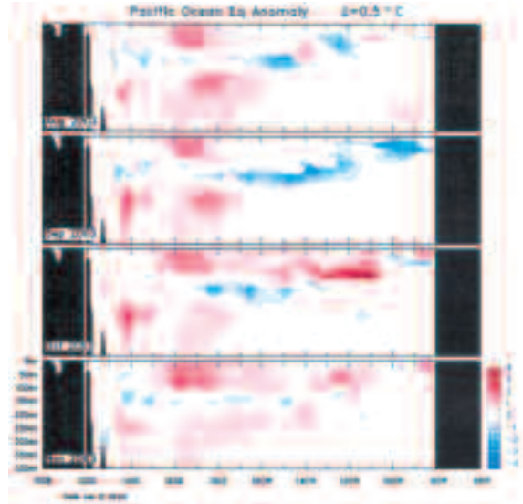
Fig. 6 Four month August to November 2003 sequence of vertical temperature anomalies at the equator. Contour interval is 0.5^{\circ}\text{C} .
