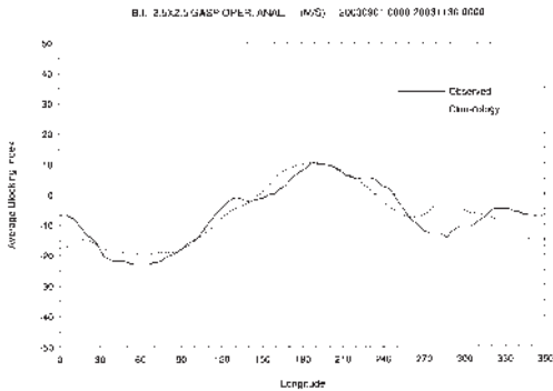
Fig. 12 Mean southern hemisphere blocking index for spring 2003 (bold line). The dashed line shows the corresponding long-term average. The horizontal axis shows the degrees east of the Greenwich meridian.
