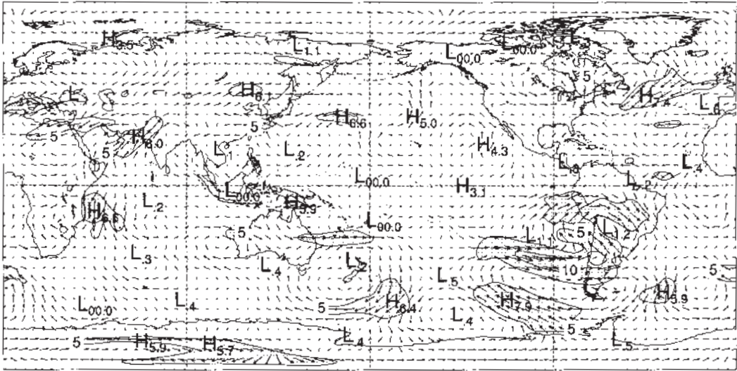
Fig. 14 Spring 2003 200 hPa vector wind anomalies with contours of vector magnitude overlaid. The contour interval is 5 \text{ m s}^{-1} , with values above 5 \text{ m s}^{-1} stippled.
