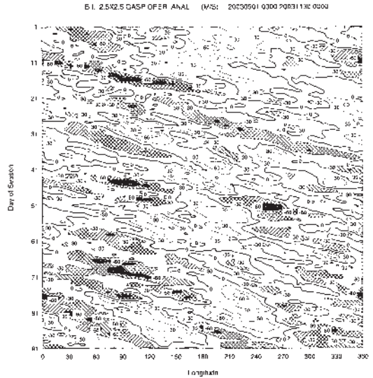
Fig. 11 Spring 2003 daily blocking index: time-longitude section. Day 1 is 1 September.
