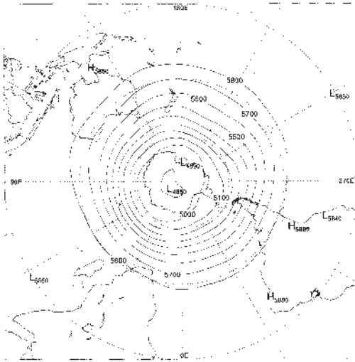
Fig. 9 Mean 500 hPa geopotential heights for spring 2003 (gpm).
