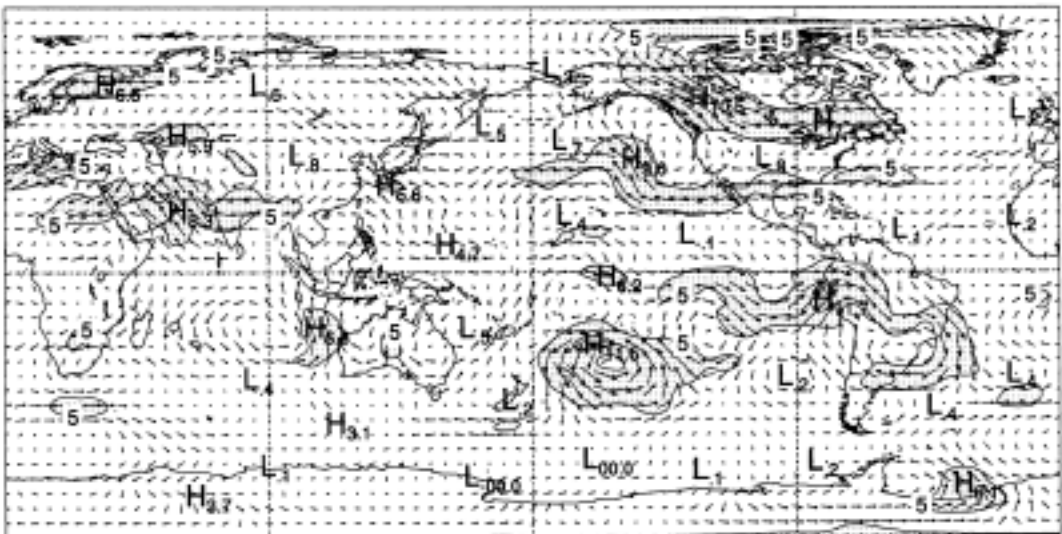
Fig. 13 Autumn 2004 200 hPa vector wind anomalies with contours of vector magnitude overlaid. The contour interval is 5 \text{ m s}^{-1} , with values above 5 \text{ m s}^{-1} stippled.
