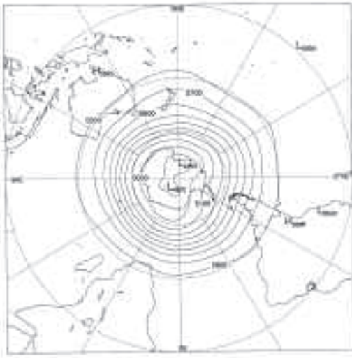
Fig. 8 Mean 500 hPa geopotential heights for autumn 2004 (gpm).
