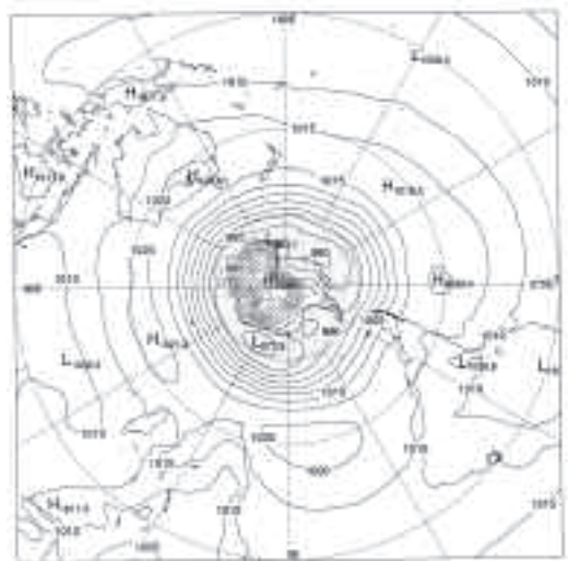
Fig. 6 Mean sea-level pressure for autumn 2004 (hPa).
