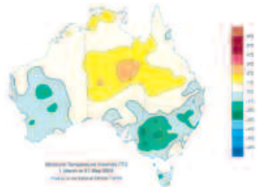
Fig. 17 Autumn 2004 minimum temperature anomalies for Australia based on a 1961-90 mean (°C).
