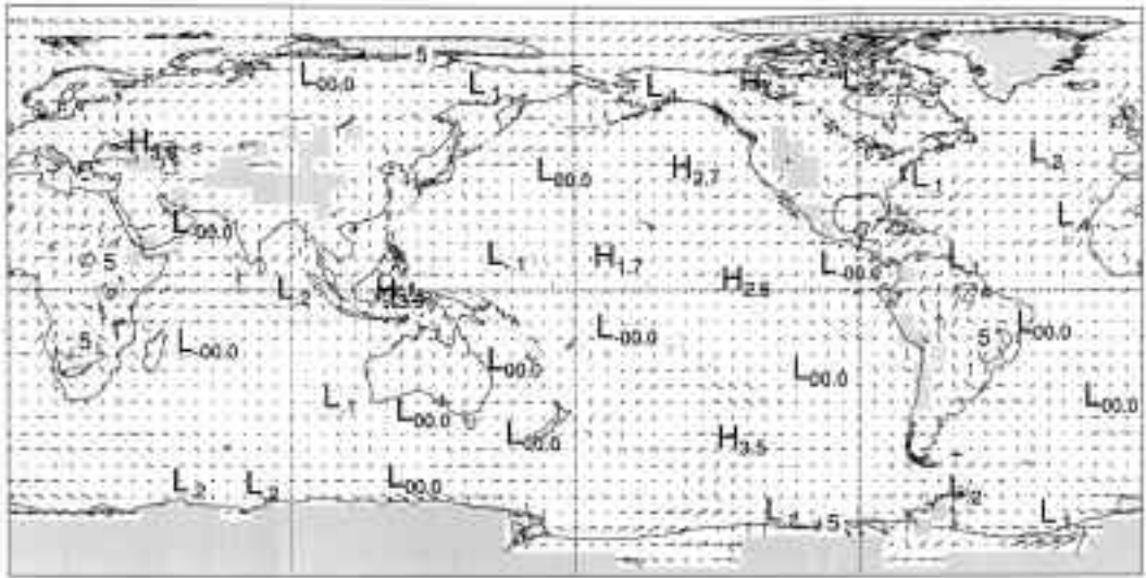
Fig. 12 Autumn 2004 850 hPa vector wind anomalies with contours of vector magnitude overlaid. The contour interval is 5 \text{ m s}^{-1} , with values above 5 \text{ m s}^{-1} stippled.
