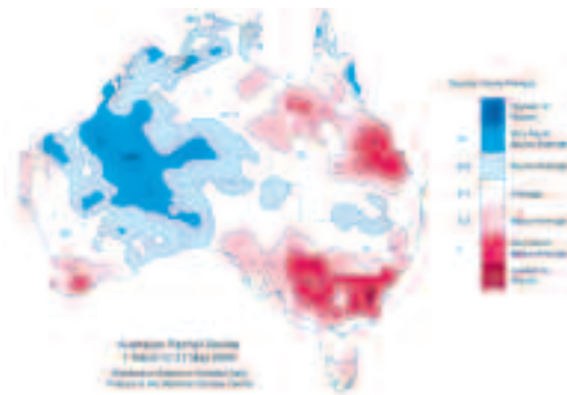
Fig. 15 Autumn 2004 rainfall deciles for Australia: decile range based on grid-point values over the autumn periods from 1900 to 2004.
