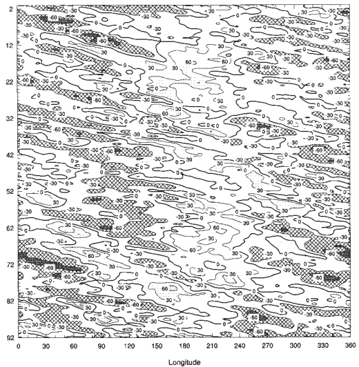
Fig. 10 Autumn 2005 daily blocking index: time-longitude section. Day 1 is 1 March.
