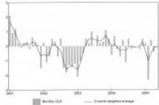
Fig. 2 Standardised anomaly of monthly outgoing long wave radiation averaged over 5°N-5°S and 160°E-160°W, for January 2001 to May 2005 inclusive. Negative (positive) anomalies indicate enhanced (reduced) convection and rainfall. Anomalies are based on a 1979-95 base period. After CPC (2005).
