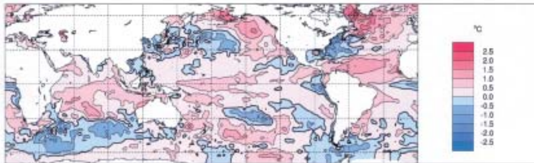
Fig. 3 Anomalies of sea-surface temperature for autumn 2005 (°C).
