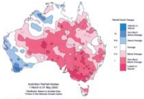
Fig 15 Autumn 2005 rainfall deciles for Australia: decile range based on grid-point values over the autumn periods from 1900 to 2005.
