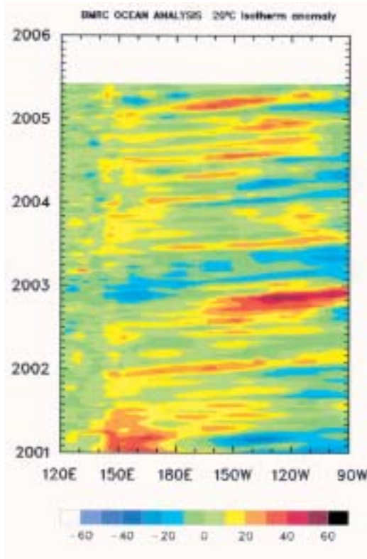
Fig. 4 Time-longitude section of the monthly anomalous depth of the 20°C isotherm at the equator for January 2001 to May 2005. Base period: 1979-89. Contour interval is 10 m.
