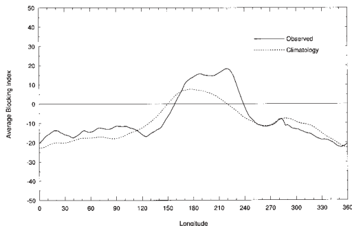
Fig. 11 Mean southern hemisphere blocking index for autumn 2005 (bold line). The dashed line shows the corresponding long-term average. The horizontal axis shows the degrees east of the Greenwich meridian.
