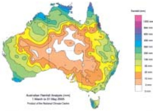
Fig. 14 Autumn 2005 rainfall totals over Australia (mm).
