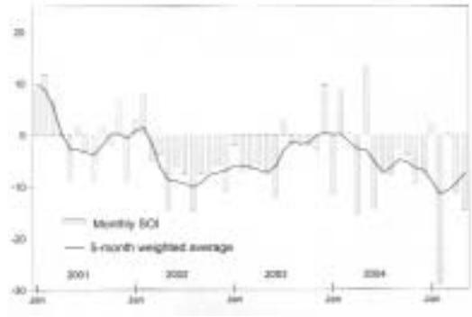
Fig. 1 Southern Oscillation Index, January 2001 to May 2005 inclusive. A curve of five-month moving averages has been superimposed on the graph. Means and standard deviations based on the period 1933-92.
