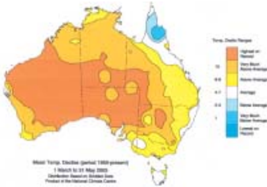
Fig. 18 Autumn 2005 mean temperature deciles for Australia: decile range based on grid-point values over the autumn periods from 1950 to 2005.
