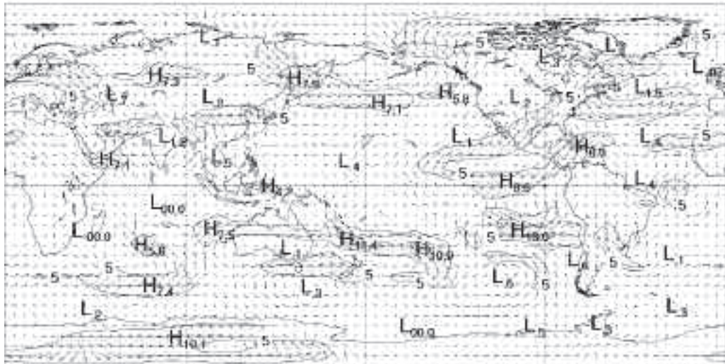
Fig. 14 Summer 2006-07 200 hPa vector wind anomalies ( \text{m s}^{-1} ).
