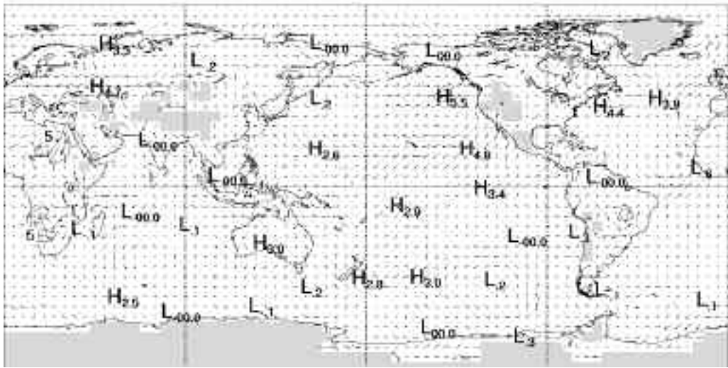
Fig. 13 Summer 2006-07 850 hPa vector wind anomalies ( \text{m s}^{-1} ).
