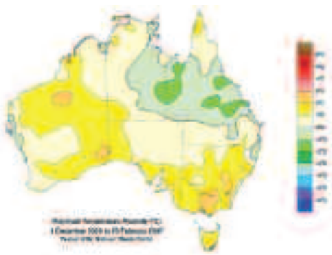
Fig. 17 Summer 2006-07 maximum temperature anomalies (°C) for Australia, based on a 1961-1990 mean.
