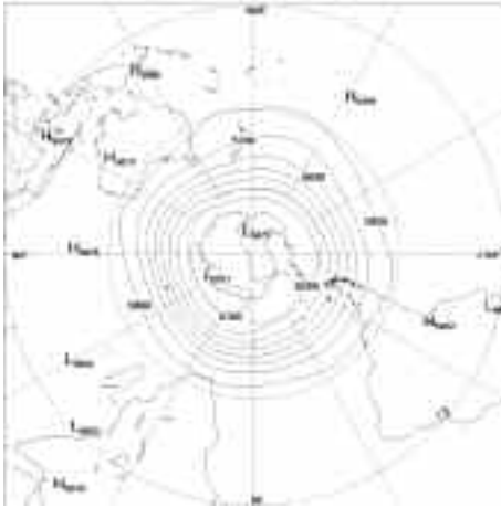
Fig. 9 Summer 2006-07 500 hPa mean geopotential height (gpm). The contour interval is 100 gpm.
