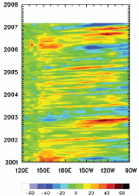
Fig. 5 Time-longitude section of the monthly anomalous depth of the 20°C isotherm at the equator from January 2001 to February 2007. The contour interval is 10 m.
