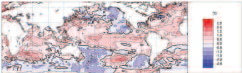
Fig. 4 Anomalies of SST for summer 2006-07 ( ^{\circ}C ). The contour interval is 0.5^{\circ}C .
