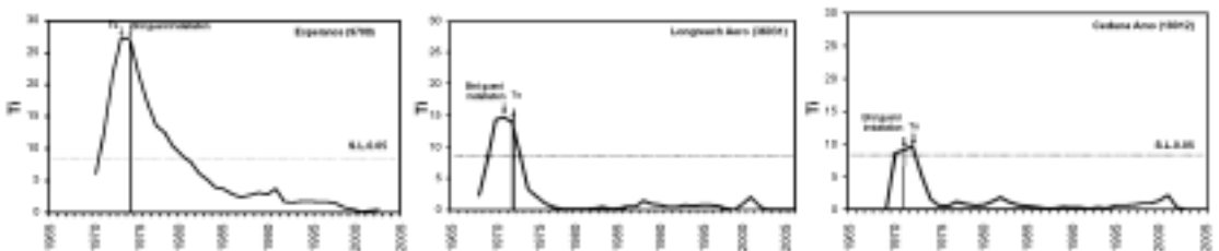
Fig. 2 Plots of T_i for selected stations for which the discontinuity ( T_0 ) is significant and close to the time of the bird guard installation. The dotted line represents the 0.05 critical level, and the vertical lines mark the times when the bird guards were installed.
