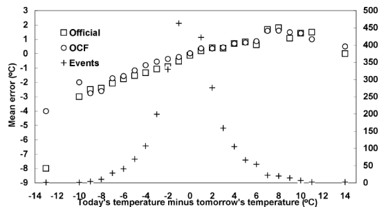
Fig. 6 As Fig. 2 but for minimum temperatures.
