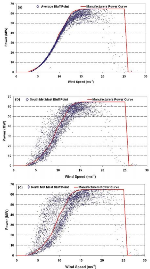
Fig. 6 Power curves for the averages of (a) The Bluff Point wind farm for August 2005, (b) The south met mast for Bluff Point for August 2005 and (c) The north met mast for Bluff Point for August 2005. The solid line in (a), (b), and (c) represents the manufacturers power curve.
