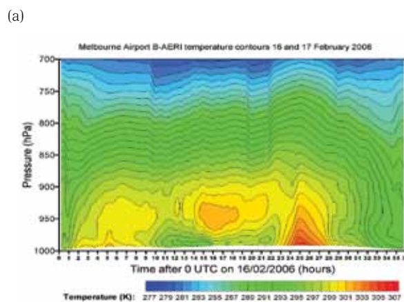
Fig. 4 (a) B-AERI time-height temperature cross-sections measured at Melbourne Airport on 16 and 17 February 2006 and (b) the MSLP analysis valid for 0000 UTC 17 February 2006.
