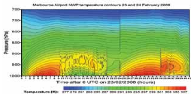
Fig. 6 Time-height temperature cross-sections used as the first guess for B-AERI time-height temperature cross-sections for Melbourne Airport from 0000 UTC 23 February to 1400 UTC 24 February 2006. These were derived from surface data and the Bureau of Meteorology Meso-LAPS model initialised at 0000 UTC 23 and 24 February 2006 and post-processed every hour.
