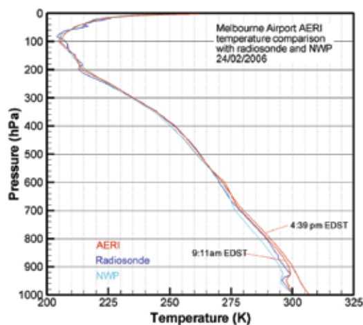
Fig. 3 The B-AERI temperature profiles at 9:11 am EDST and 4:39 pm EDST, the radiosonde profile at 9:00 am EDST and the NWP first guess profile at 9:11 am EDST for Melbourne Airport on 24 February 2006.
