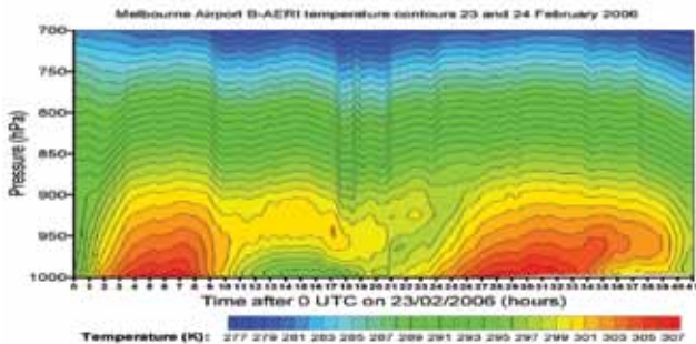
Fig. 5 B-AERI time-height temperature cross-sections measured at Melbourne Airport from 0000 UTC 23 February to 1400 UTC 24 February 2006.
