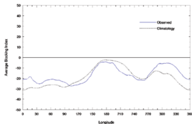
Fig. 12 Mean southern hemisphere blocking index ( \text{m s}^{-1} ) for summer 2008-09 (solid line). The dashed line shows the corresponding long-term average. The horizontal axis shows degrees east of the Greenwich meridian.
