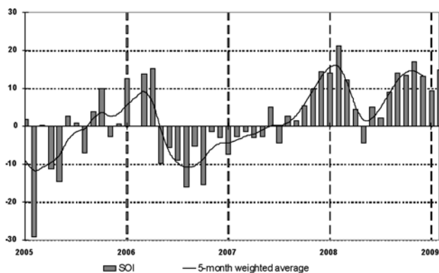
Fig. 1 Southern Oscillation Index, from January 2005 to February 2009, together with a five-month binomially weighted moving average. Means and standard deviations used in the computation of the SOI are based on the period 1933-1992.
