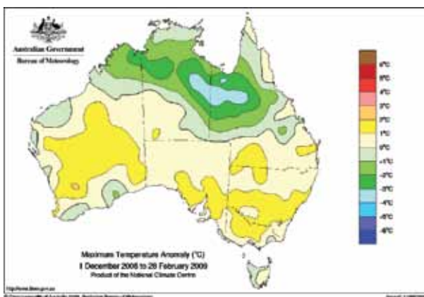
Fig. 17 Summer 2008-09 maximum temperature anomalies (°C) for Australia.
