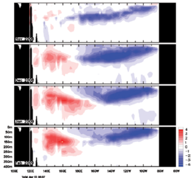
Fig. 6 Four-month November 2008 to February 2009 sequence of vertical temperature anomalies at the equator for the Pacific Ocean. The contour interval is 0.5°C.
