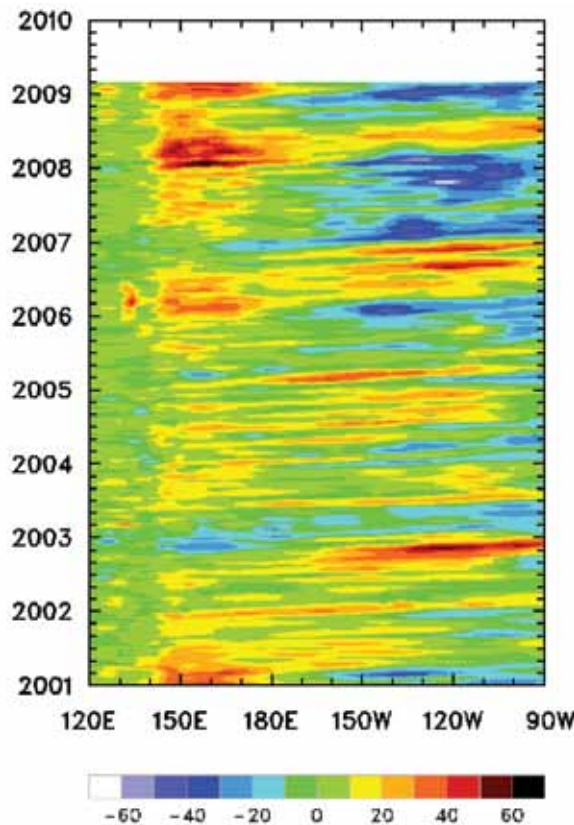
Fig. 5 Time-longitude section of the monthly anomalous depth of the 20°C isotherm at the equator for January 2001 to February 2009. The contour interval is 10 m.
