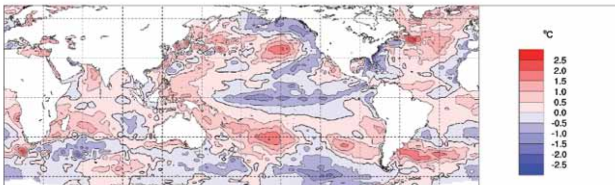
Fig. 4 Anomalies of SST for summer 2008-09 ( ^{\circ}C ). The contour interval is 0.5^{\circ}C .
