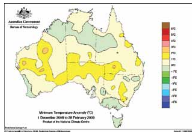
Fig. 18 Summer 2008-09 minimum temperature anomalies (°C) for Australia.
