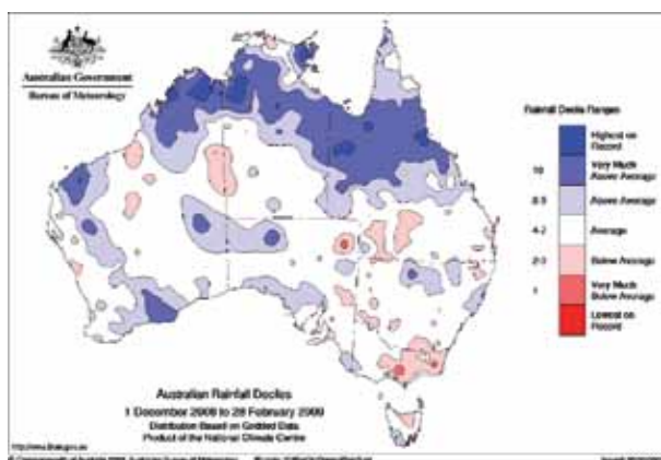
Fig. 16 Summer 2008-09 rainfall deciles for Australia. Decile ranges based on grid-point values over the summers 1900-01 to 2008-09.
