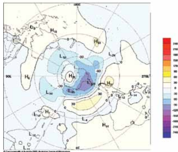
Fig. 10 Summer 2008-09 500 hPa mean geopotential height anomaly (gpm).
