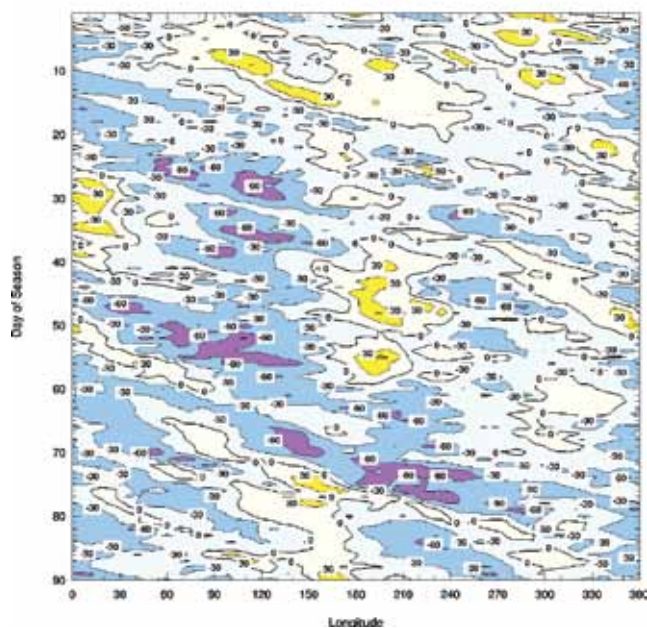
Fig. 11 Summer 2008-09 daily southern hemisphere blocking index ( \text{m s}^{-1} ) time-longitude section. The horizontal axis shows degrees east of the Greenwich meridian. Day one is 1 December 2008.
