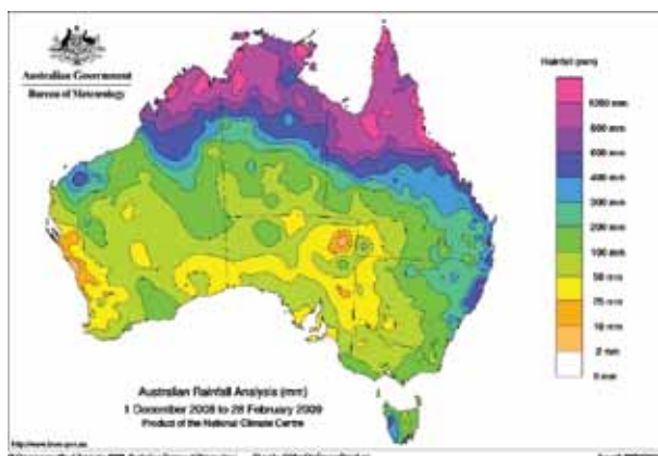
Fig. 15 Summer 2008-09 rainfall totals (mm) for Australia.
