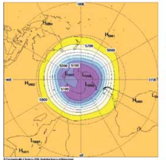
Fig. 9 Summer 2008-09 500 hPa mean geopotential height (gpm).
