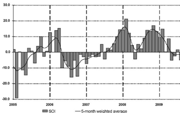
Fig. 1 Southern Oscillation Index from January 2005 to August 2009, together with a five-month binomially weighted moving average. Means and standard deviations used in the computation of the SOI are based on the period 1933-1992.
