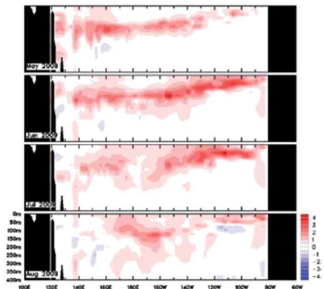
Fig. 7 Four-month (May to August 2009) sequence of vertical temperature anomalies at the equator for the Pacific Ocean. The contour interval is 0.5°C.
