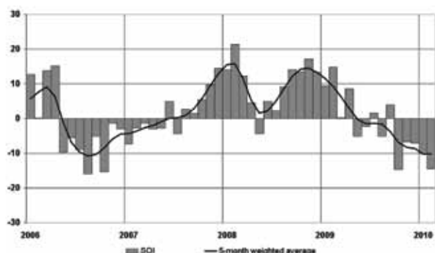
Fig. 1 Southern Oscillation Index (SOI), from January 2006 to February 2010, together with a five-month binomially weighted moving average. Means and standard deviations used in the computation of the SOI are based on the period 1933–1992
