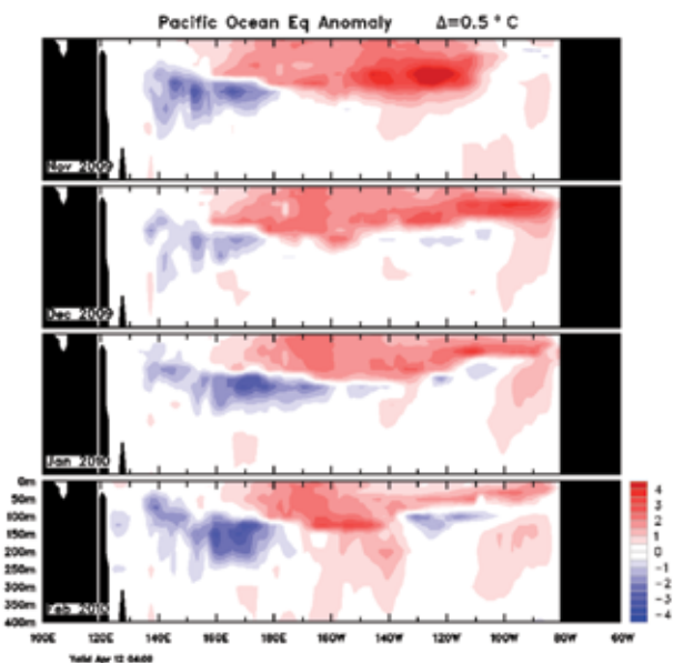
Fig. 6 Four-month November 2009 to February 2010 sequence of vertical sea subsurface temperature anomalies at the equator for the Pacific Ocean. The contour interval is 0.5 °C.
