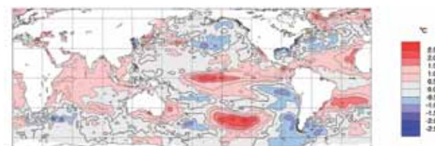
Fig. 4 Anomalies of SST for summer 2009–2010 (°C). The contour interval is 0.5 °C.
