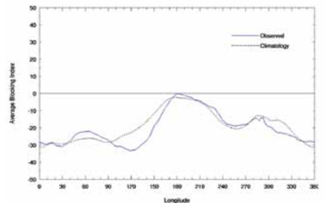
Fig. 12 Mean southern hemisphere blocking index ( ms^{-1} ) for summer 2009–2010 (solid line). The dashed line shows the corresponding long-term average. The horizontal axis shows degrees east of the Greenwich meridian.
