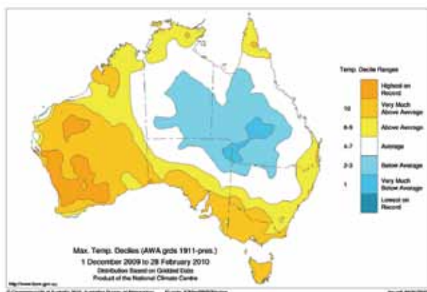
Fig. 18 Summer 2009–2010 maximum temperature deciles. Decile ranges based on grid-point values over the summers 1911–1912 to 2009–2010.
