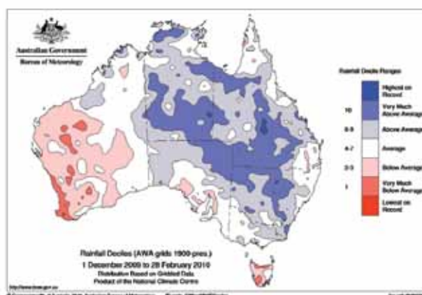
Fig. 16 Summer 2009–2010 rainfall deciles for Australia. Decile ranges based on grid-point values over the summers 1900–1901 to 2009–2010.
