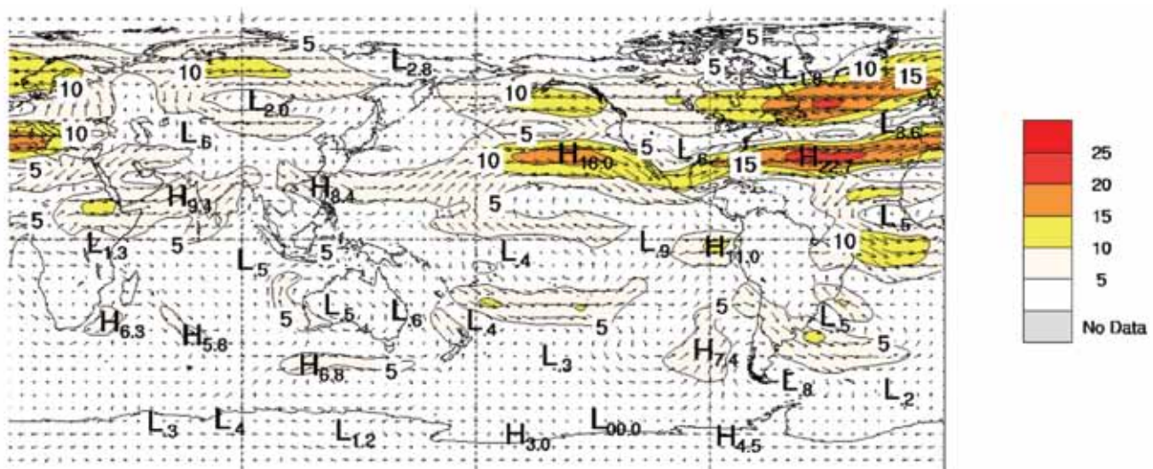
Fig. 14 Summer 2009–2010 200 hPa vector wind anomalies (ms -1 ).
