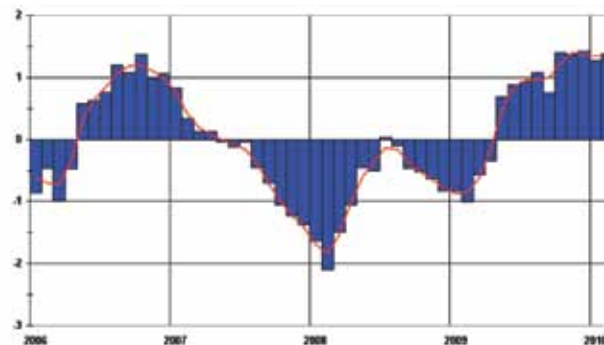
Fig. 2 Composite standardised monthly ENSO index from January 2006 to February 2010, together with a weighted three-month moving average. See text for details.
