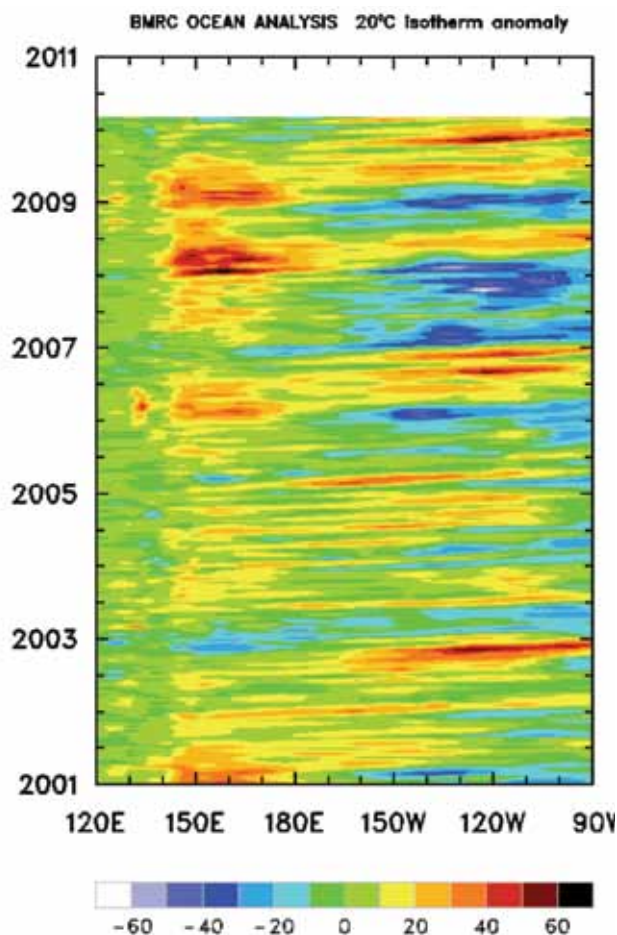
Fig. 5 Time-longitude section of the monthly anomalous depth of the 20 °C isotherm at the equator for January 2001 to February 2010. The contour interval is 10 m.
