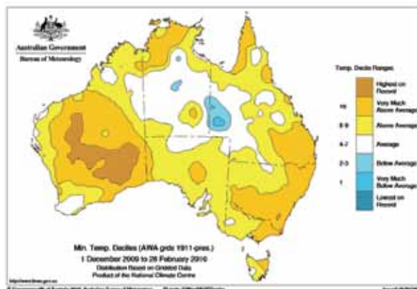
Fig. 20 Summer 2009/2010 minimum temperature deciles. Decile ranges based on grid-point values over the summers 1911–1912 to 2009–2010.
