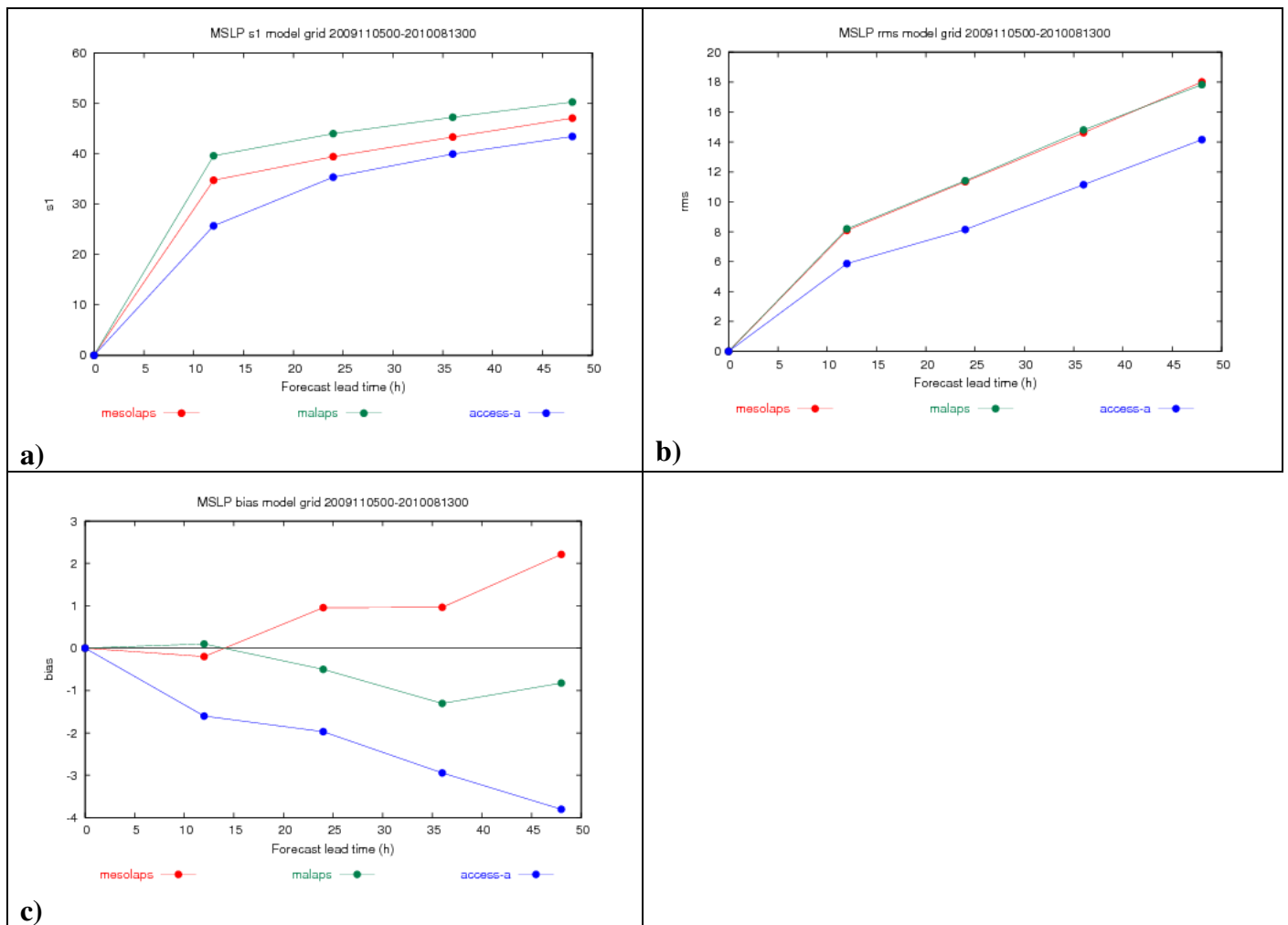
Figure 11: Verification of mesoscale model Mean Sea Level pressure forecasts for the Australian region averaged over the period 5 November 2009 to 13 August 2010 for ACCESS-A (blue), MESOLAPS (red), MALAPS (green) for a) S1 skill Score, b) RMS error, c) bias. All fields are self-verified , i.e. the forecasts from each system are compared to the system's own analysis. Calculations have been performed on the model grid , from 45°S to 10°S, and 110°E to 155°E. Vertical scale is in units of 0.1 hPa
