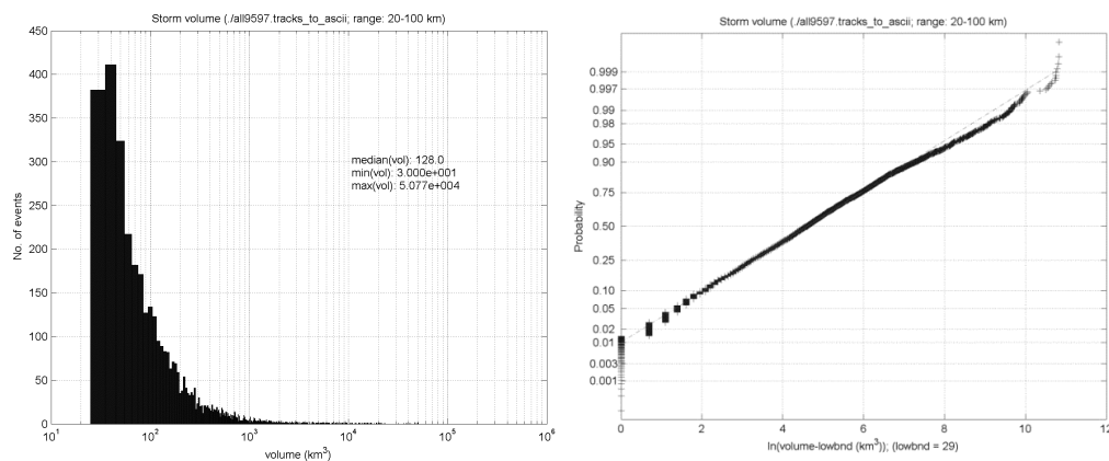
Figure 1. a) Frequency distribution for 30-dBZ storm volume. b) Normal probability plot of \ln(\text{volume}-k) .
