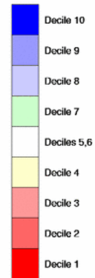
Mean Rainfall Decile Ranges
