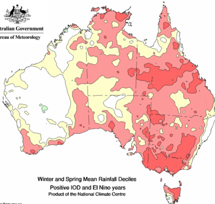
Mean Rainfall Decile Ranges
