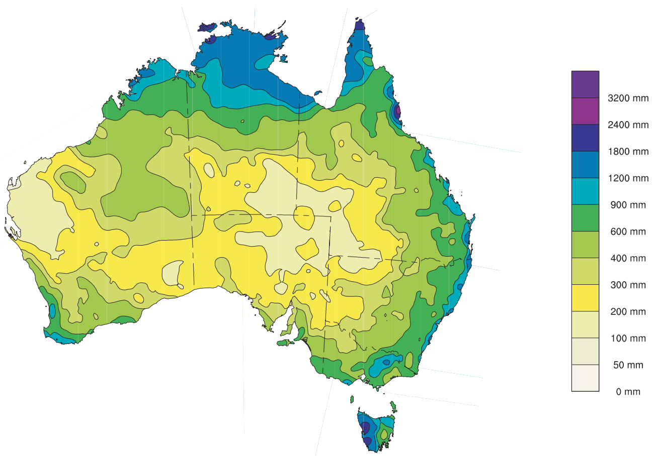
Distribution of 2003 Annual Rainfall Totals
