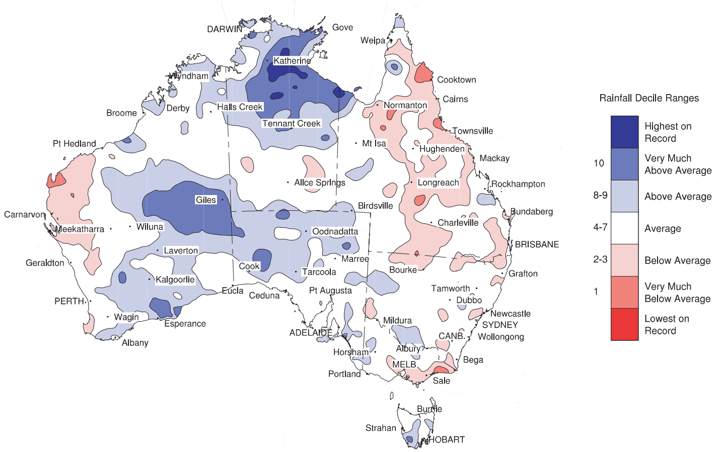
Distribution of 2003 Annual Rainfall Deciles (based on 104 year climatology of gridded fields from 1900-2003)
