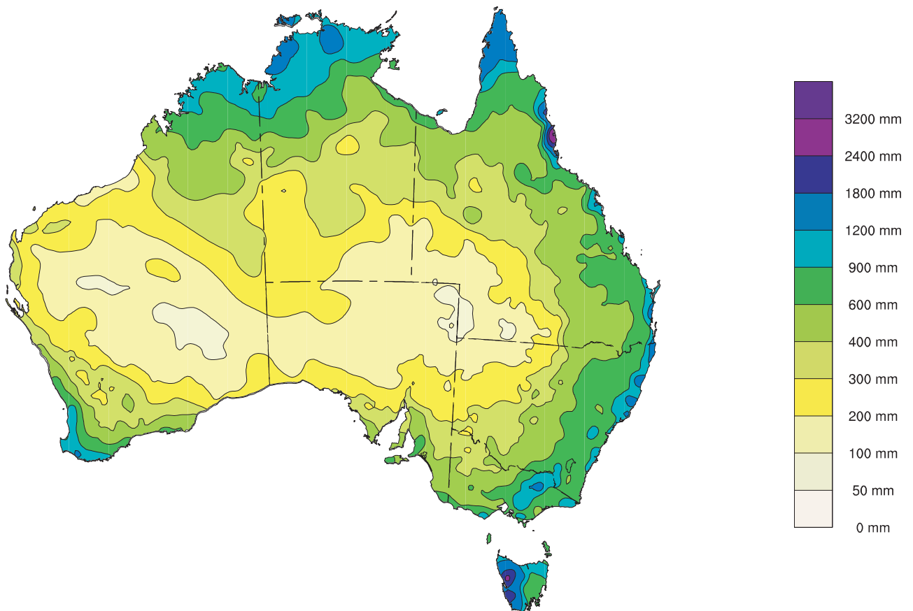
Distribution of 2005 Annual Rainfall Totals
