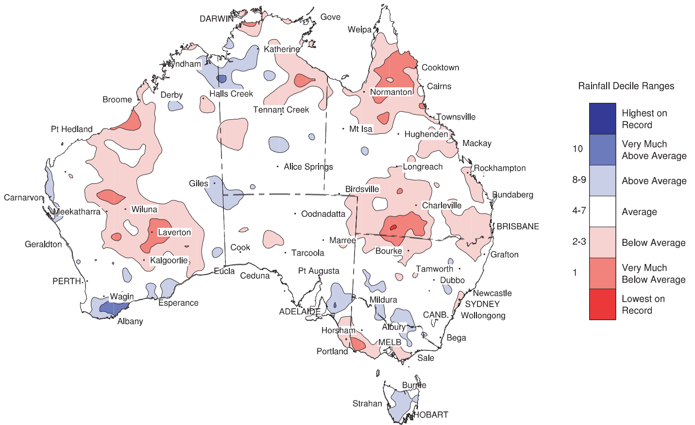
Distribution of 2005 Annual Rainfall Deciles (based on a 106 year climatology of gridded fields from 1900-2005)
