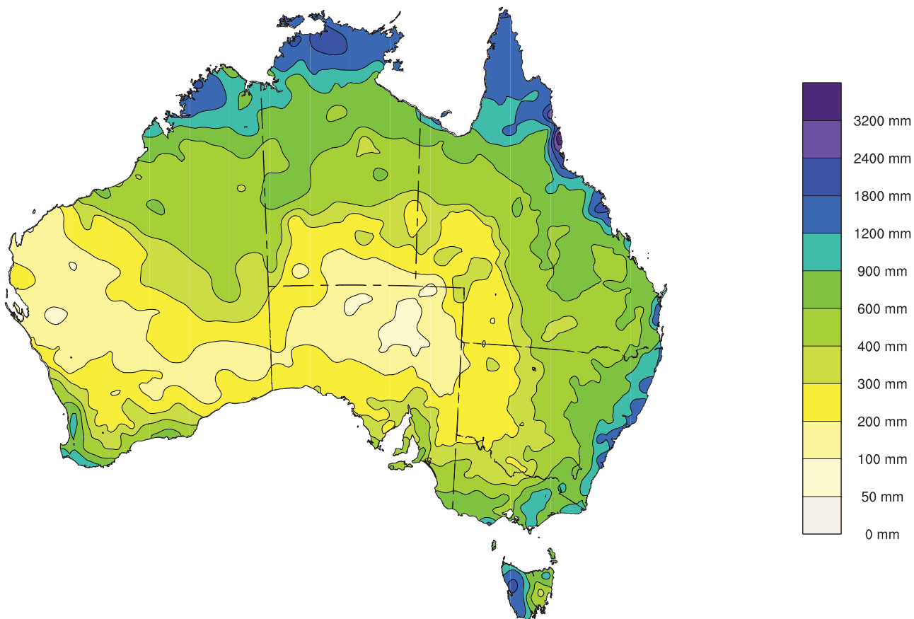
Distribution of 2007 Annual Rainfall Totals
