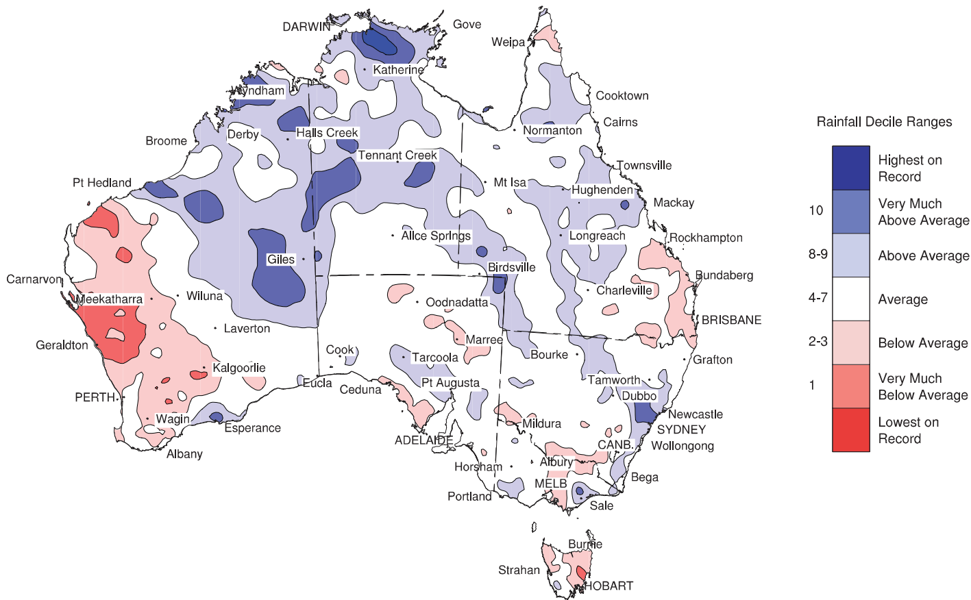
Distribution of 2007 Annual Rainfall Deciles (based on a 108-year climatology of gridded fields from 1900-2007)
