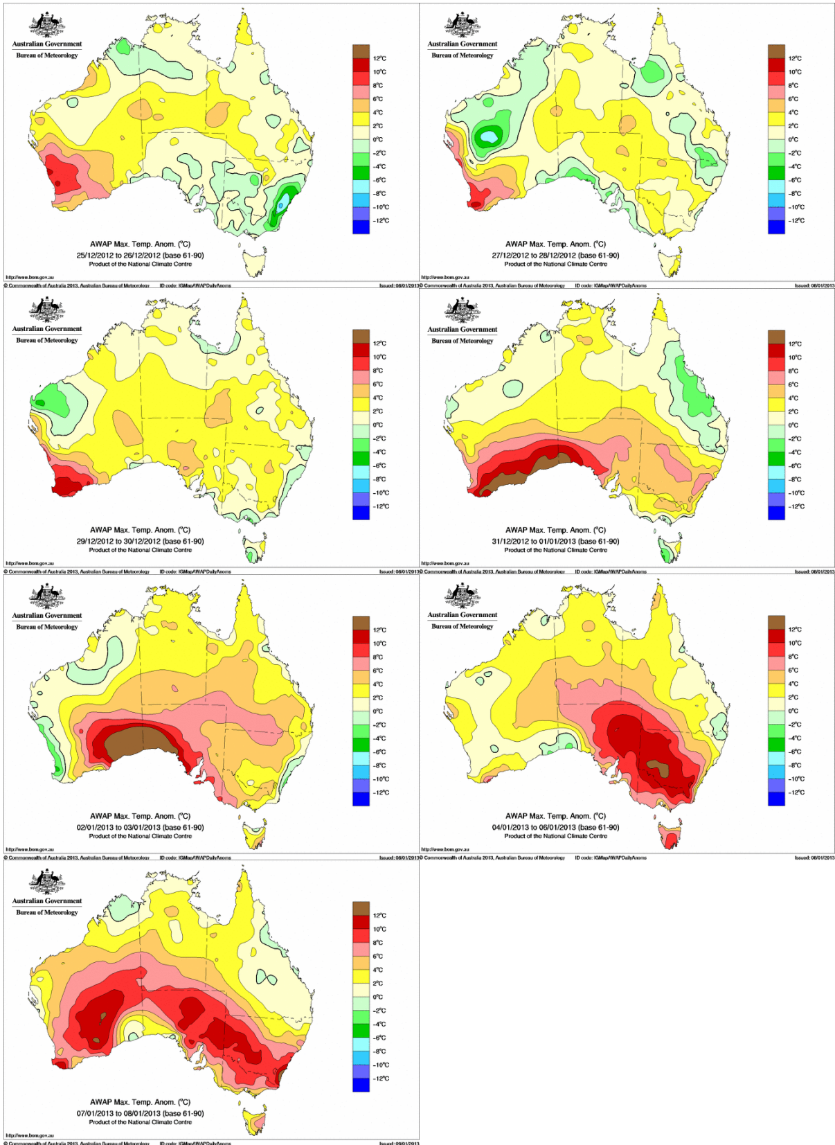
Figure 1: The maximum temperature anomaly from the 1961-1990 average for consecutive two day periods over the period 25 December 2012 to 8 Jan 2013. Units are °C.
