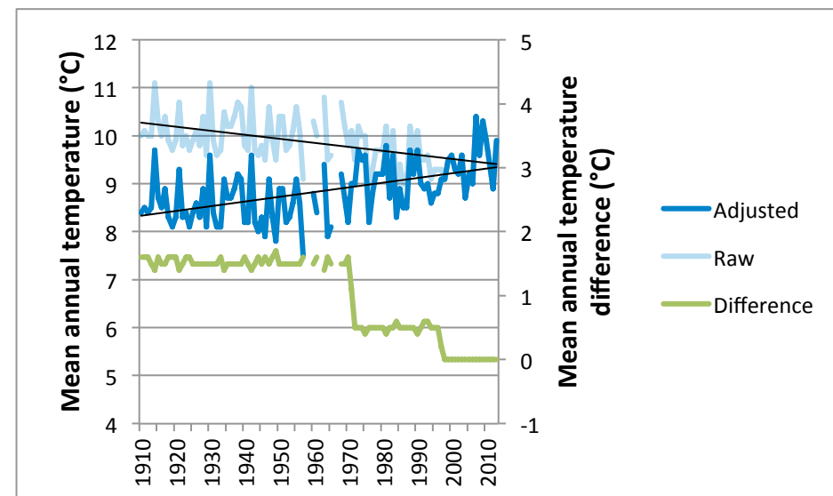
Chart 1: Deniliquin annual average minimum temperatures (1910–2013)
