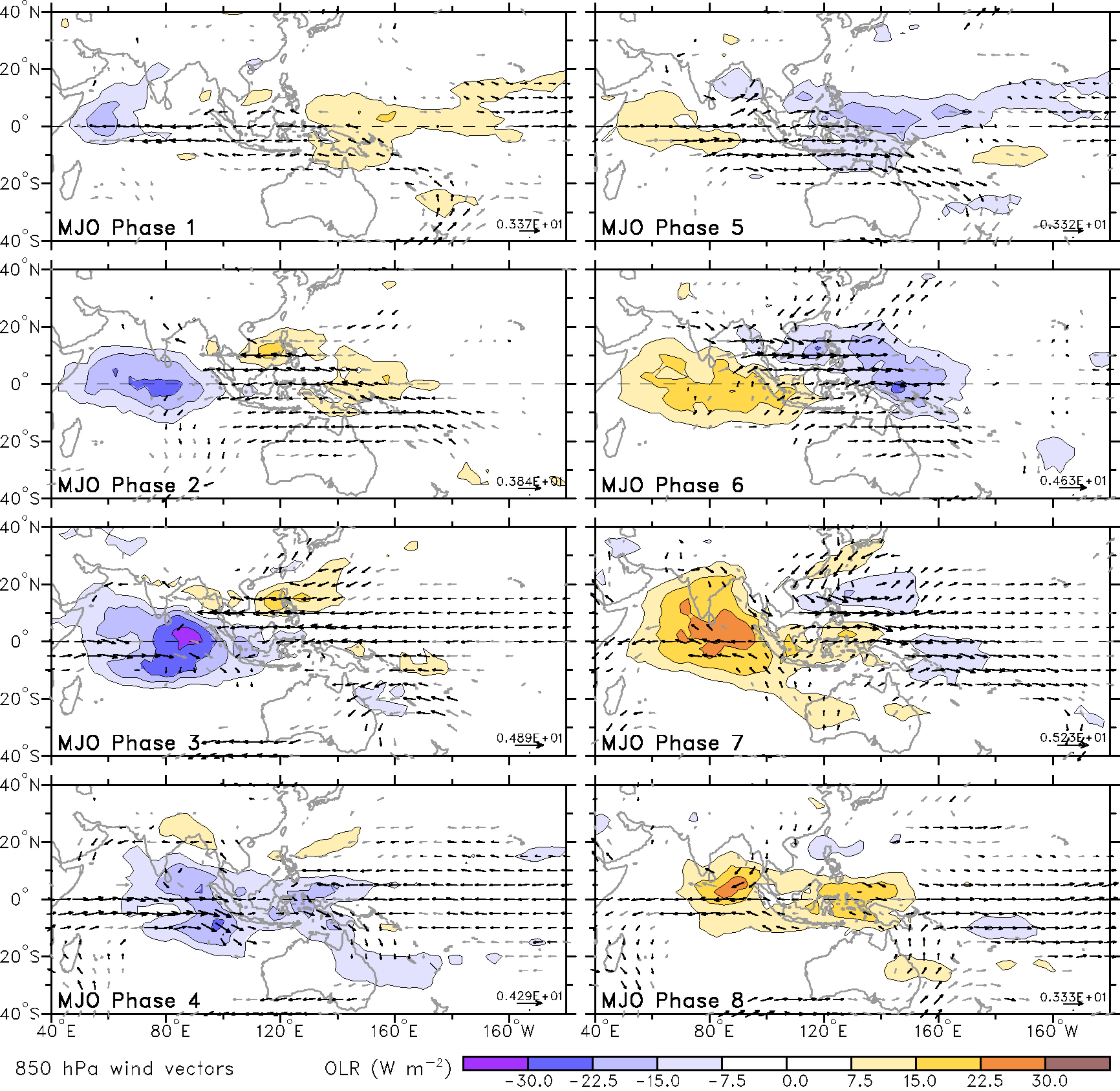
MJO average conditions in Apr-May-Jun, 1974-2009
