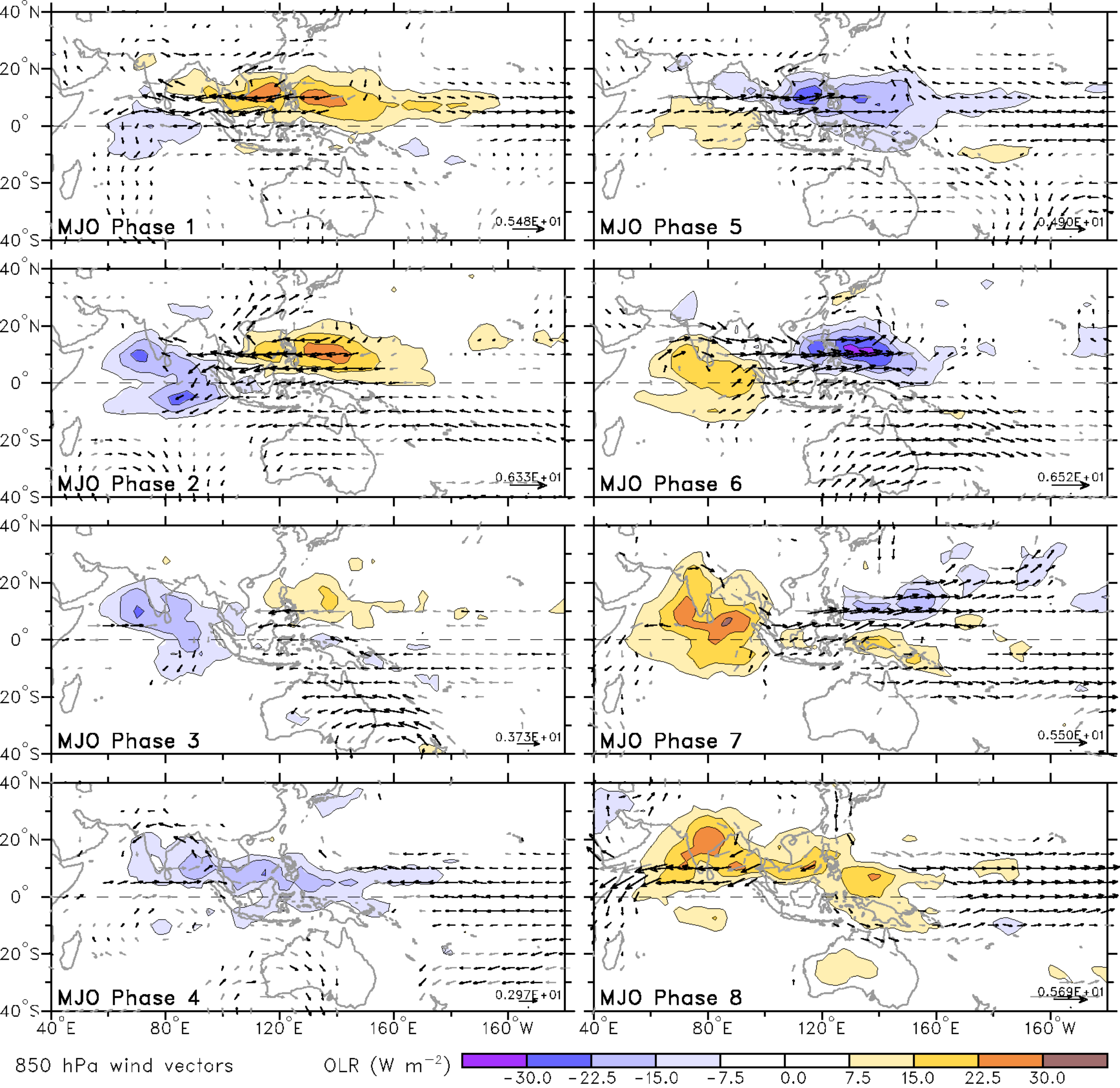
MJO average conditions in Aug-Sep-Oct, 1974-2009
