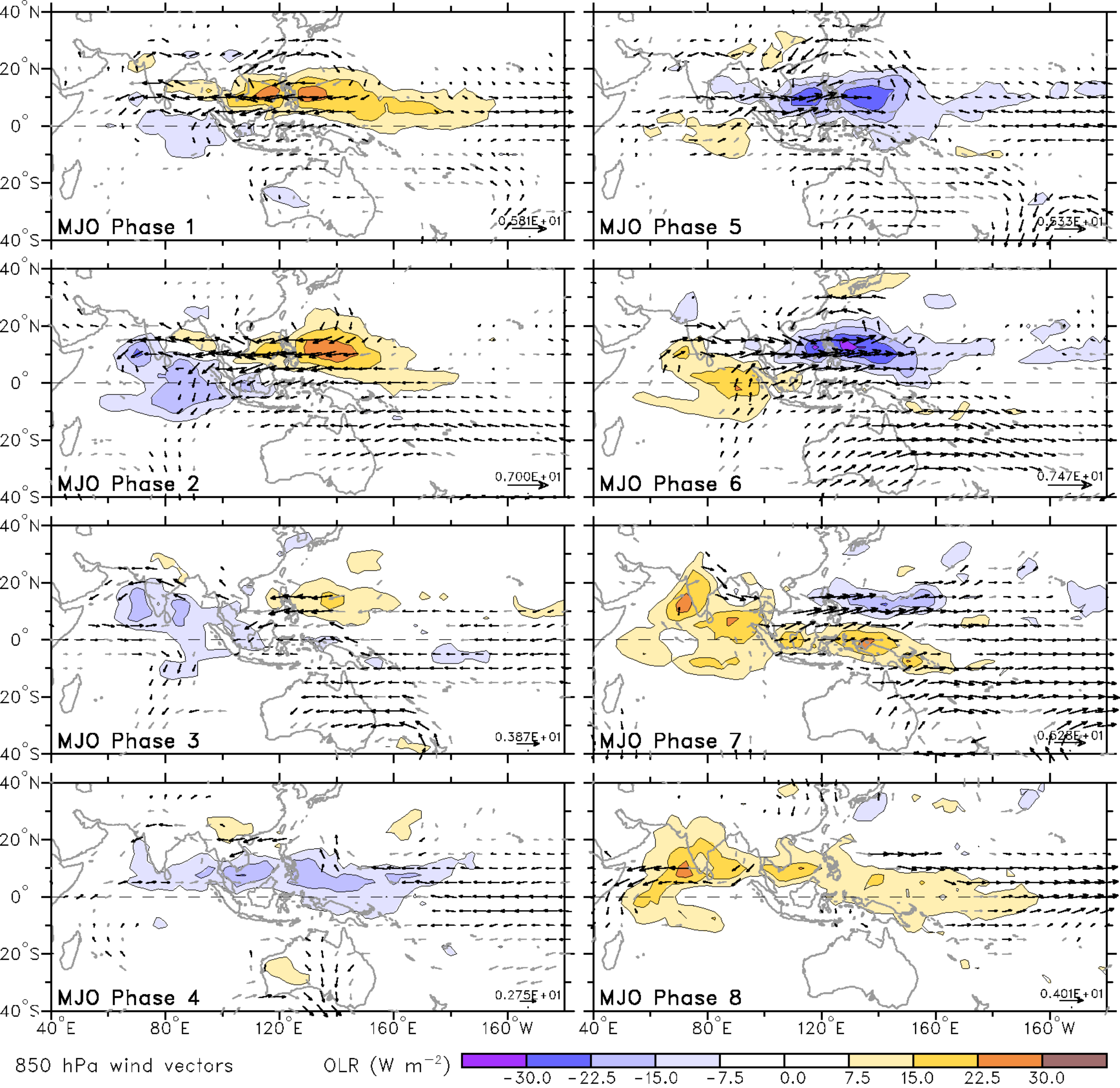
MJO average conditions in Jul-Aug-Sep, 1974-2009
