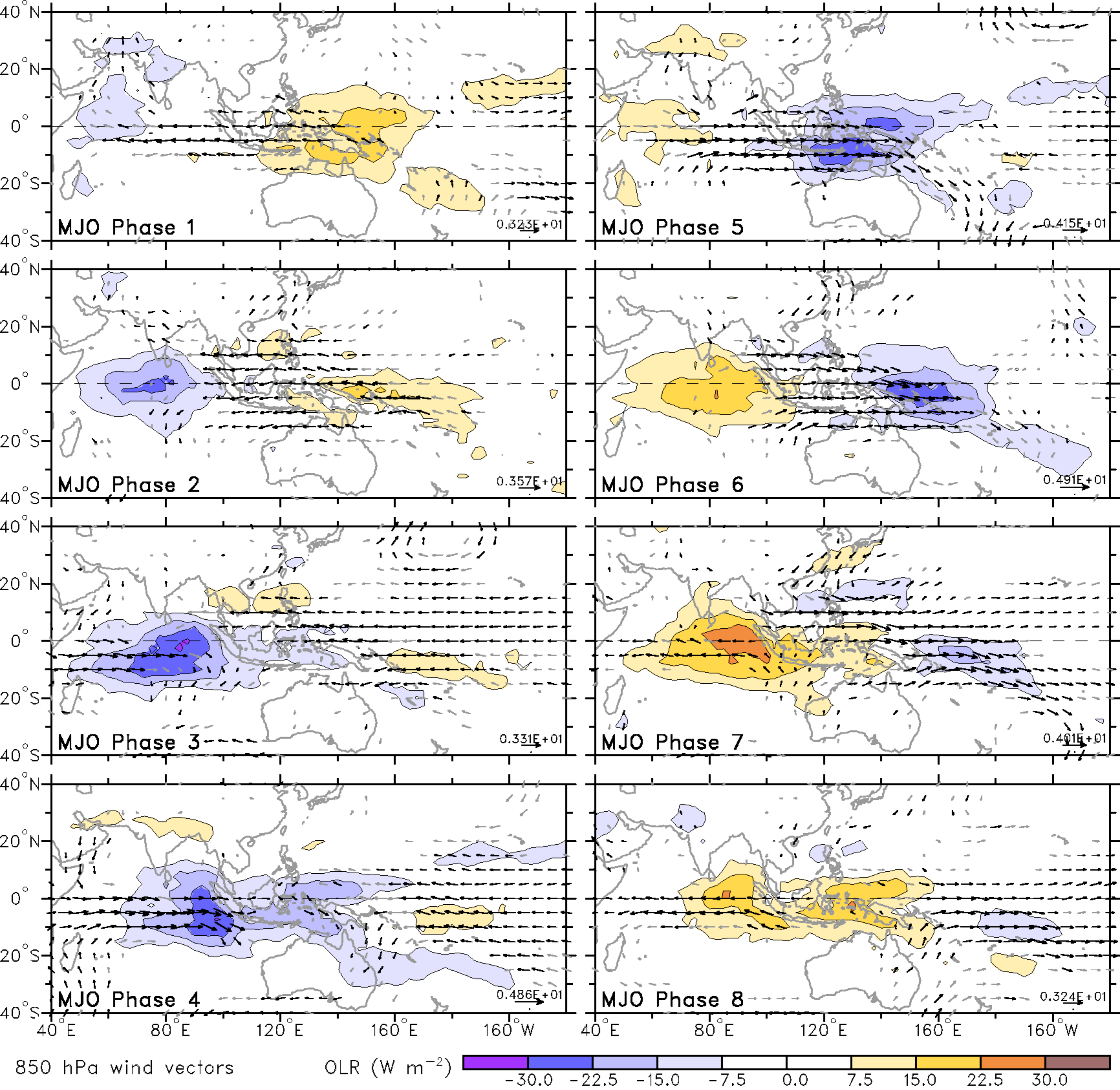
MJO average conditions in Mar-Apr-May, 1974-2009
