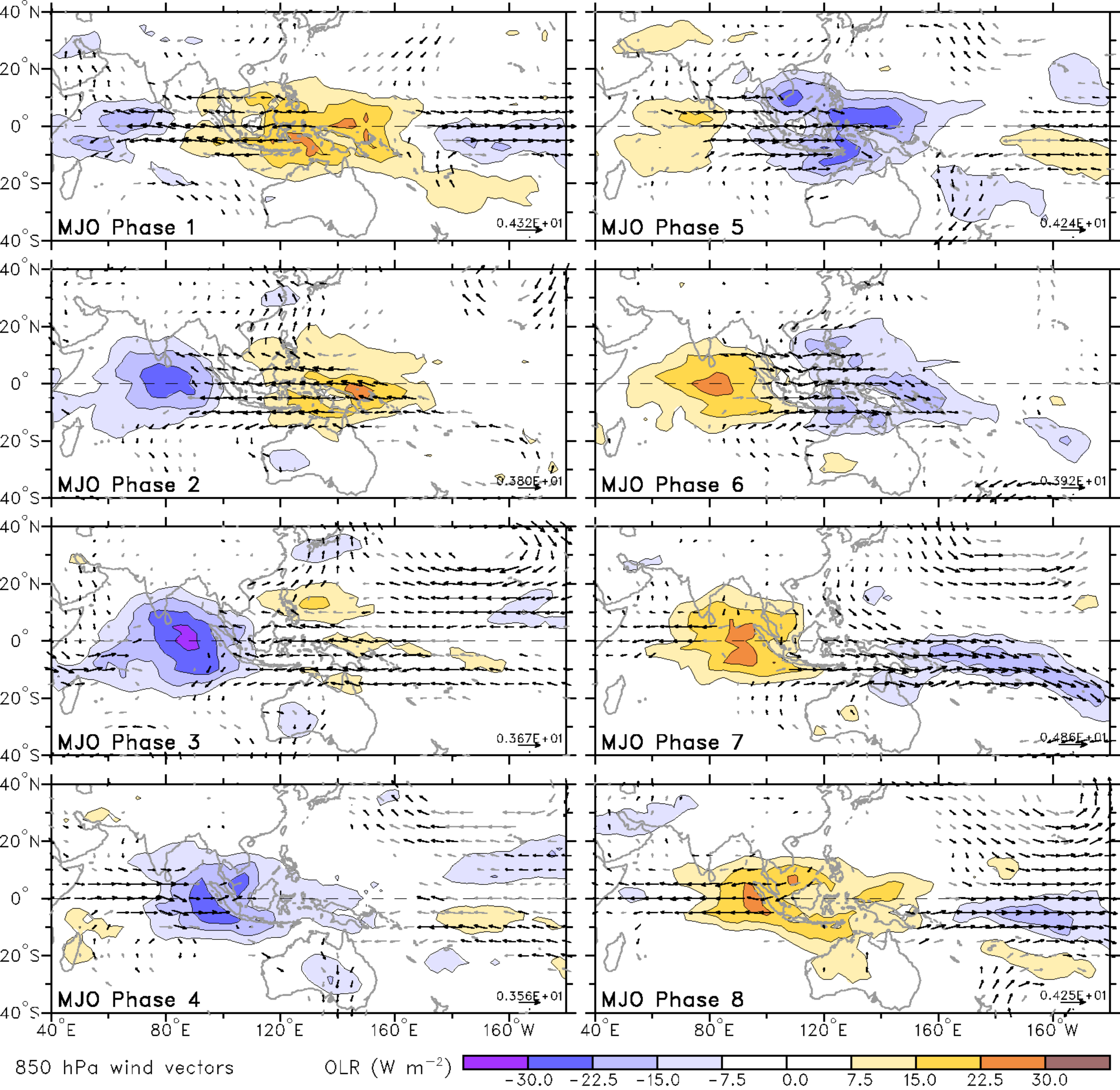
MJO average conditions in Nov-Dec-Jan, 1974-2009
