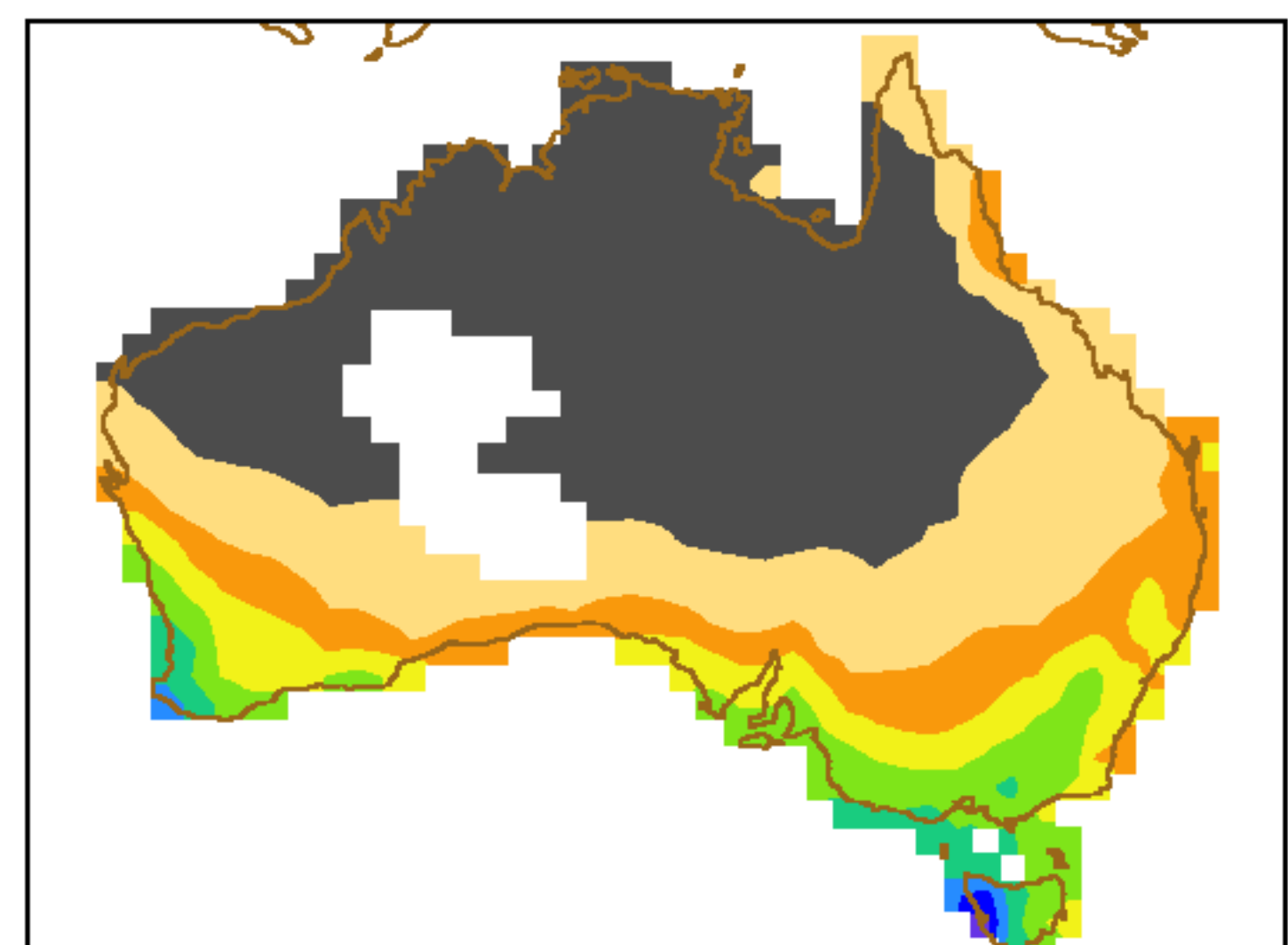
Normal weekly rainfall in JAS (mm)
