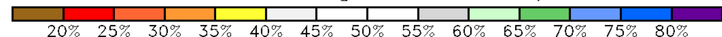
Chance of exceeding normal weekly rainfall
