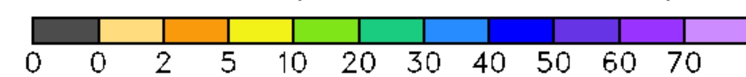
Normal weekly rainfall in JJA (mm)
