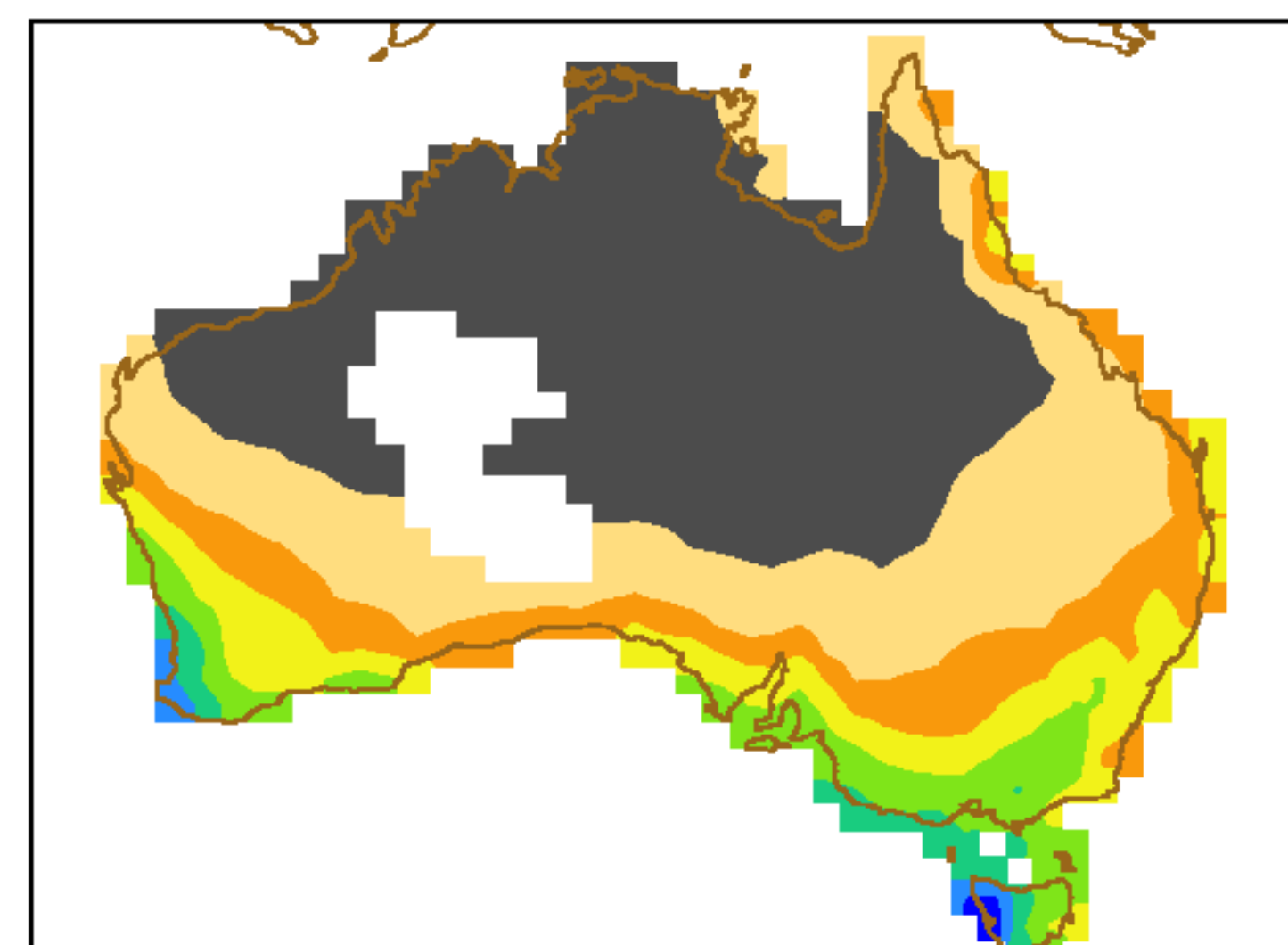
Normal weekly rainfall in JJA (mm)
