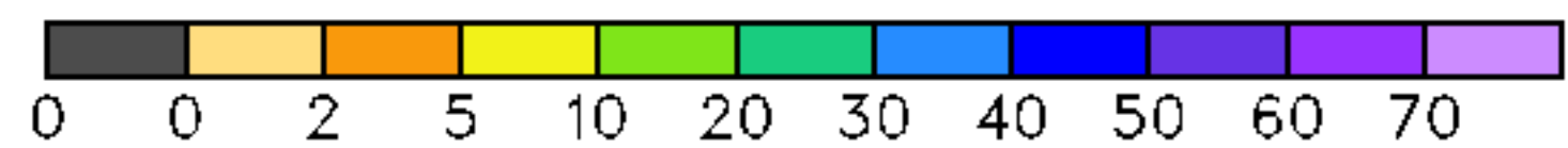
Normal weekly rainfall in MJJ (mm)
