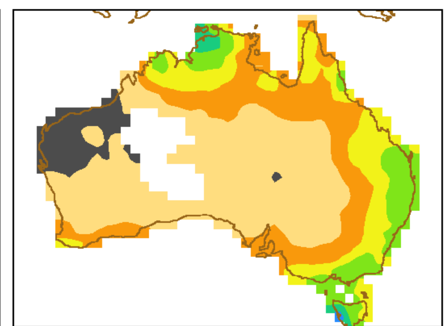
Normal weekly rainfall in OND (mm)
