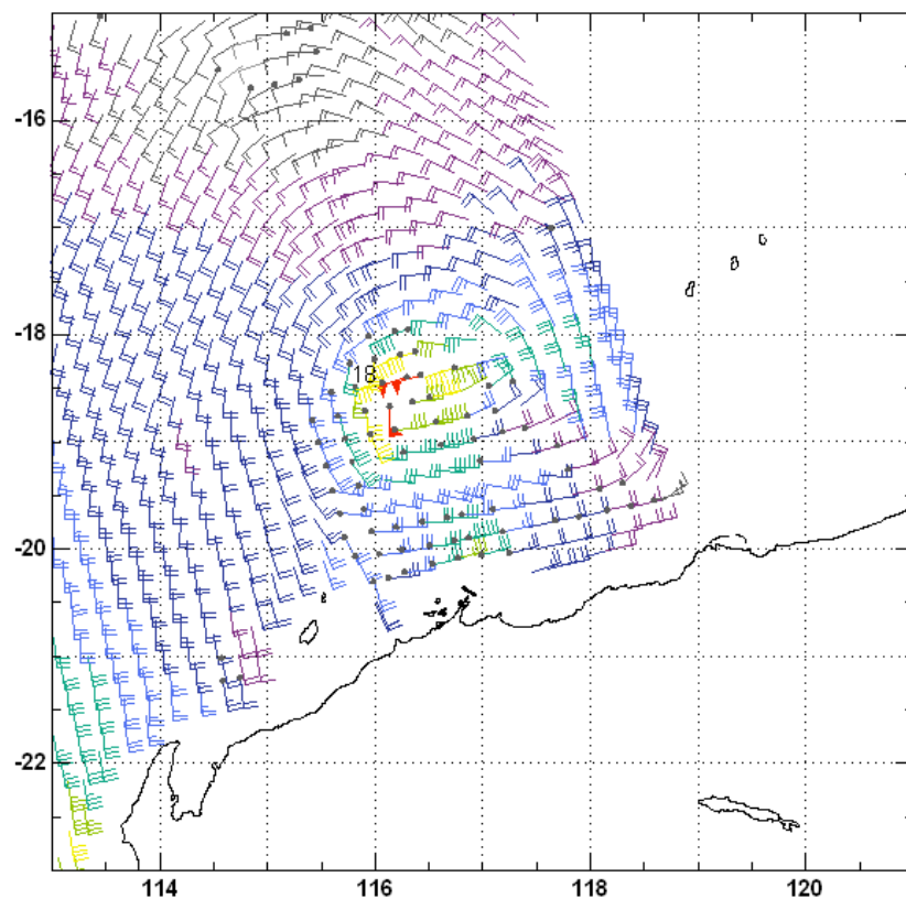
Figure 4. Quikscat at 22:55UTC 26 March 2007.
