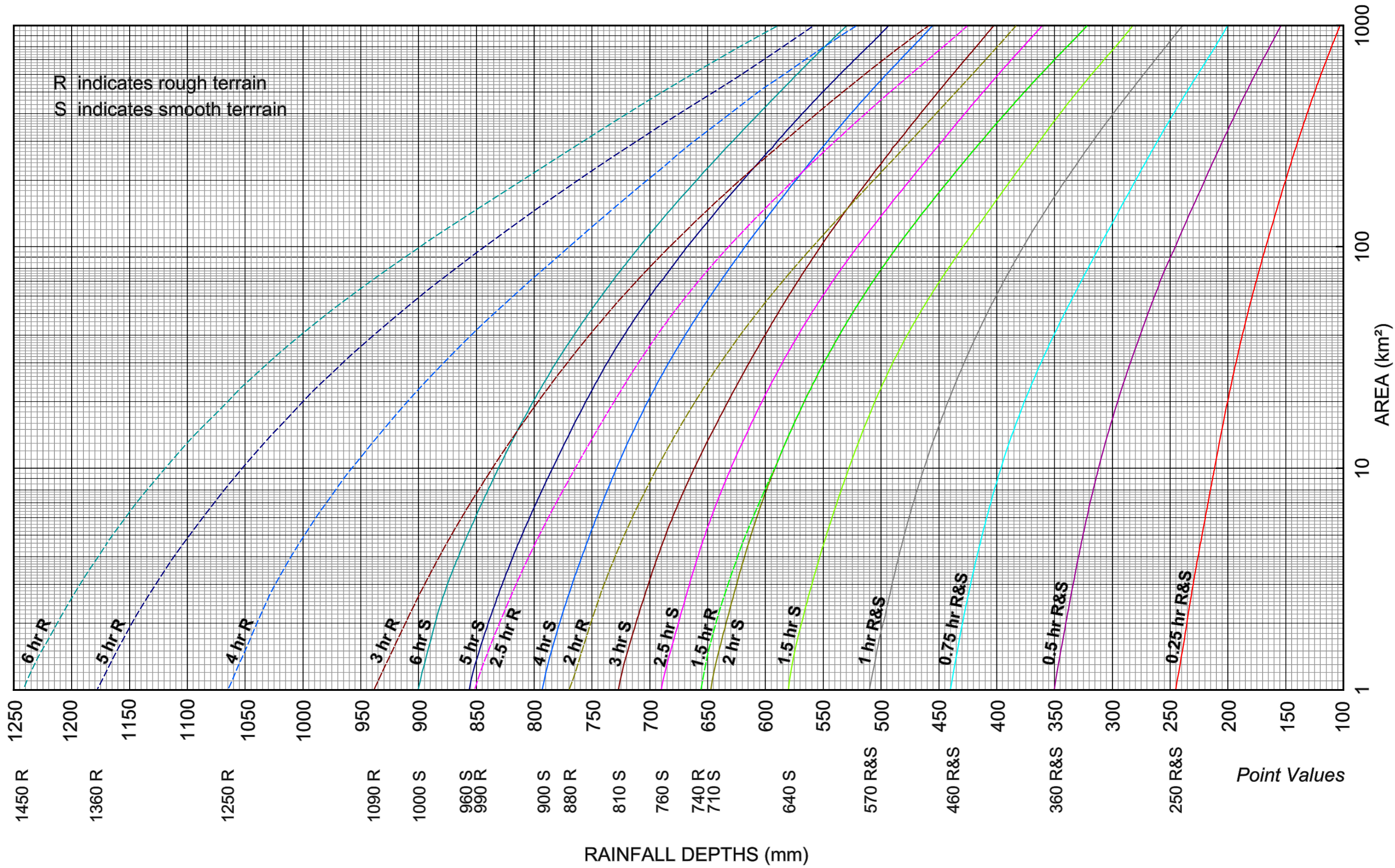
Depth-Duration-Area Curves of Short Duration Rainfall
