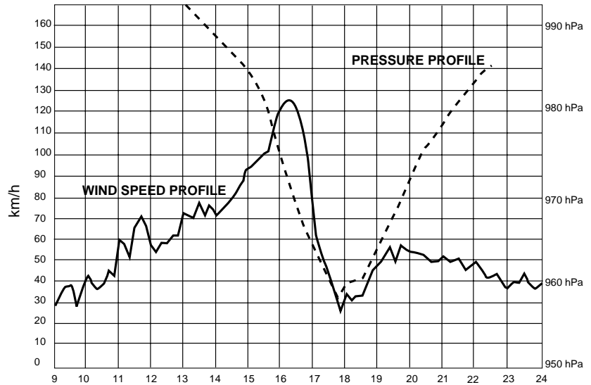
Figure 5 Typical wind speed and pressure relationships for a tropical cyclone - cyclone Winifred , Cowley Beach, Queensland, February 1986.
