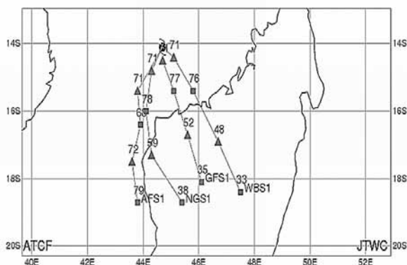
Fig. 1 STIPS ensemble members for the 26 January 1200 UTC forecast for Tropical Cyclone Fame, the 13th tropical cyclone of the 2008 JTWC season. Forecast periods are 12, 24, 36 and 48 h and each position is labeled with corresponding STIPS ensemble member intensity forecast (kn). The solid typhoon symbol represents the initial position, and the four characters at the end of each forecast indicate the specific ensemble member.
