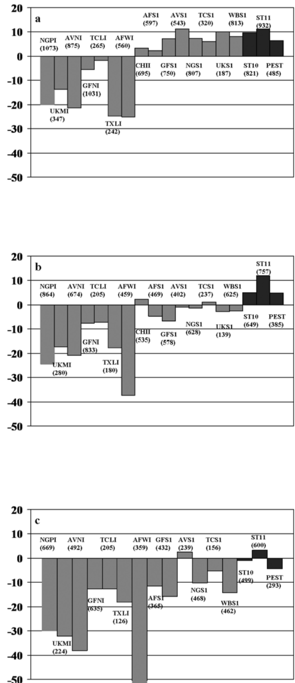
Fig. 2 Comparison of intensity forecast skill (per cent) for JTWC early forecast aids at (a) 24 h (b) 48 h and (c) 72 h. Data includes 2006-2008 southern hemisphere seasons. Skill is based on ST5D and the comparison is inhomogeneous. Acronyms are defined in Table 1 and Table A1. Number of cases is shown in parentheses. Consensus aids are shaded dark. ST11 consensus was not available to JTWC in 2006, and was recomputed for this evaluation.
