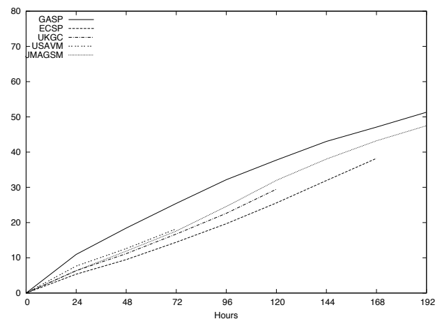
Fig. 2(b) 500 hPa geopotential height S1 skill score comparison, for different forecast periods, between GASP, ECSP, UKGC, USAVN and JMAGSM (October to December 2008).
