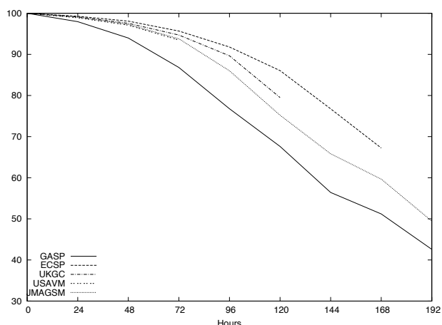
Fig. 3 Anomaly correlation of MSLP comparison, for different forecast periods, between GASP, ECSP, UKGC, USAVN and JMAGSM (October to December 2008).
