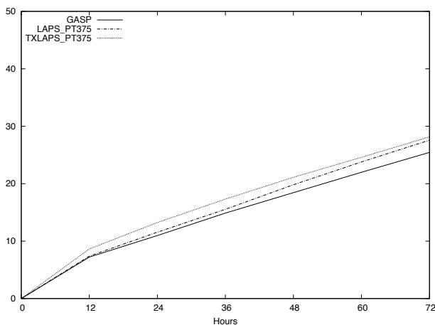
Fig. 1(b) 500 hPa geopotential height S1 skill score comparison, for different forecast periods, between GASP, LAPS_PT375, and TXLAPS_PT375 (October to December 2008).
