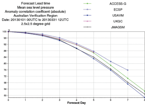
Fig. 3. Anomaly correlation of MSLP comparison, for different forecast periods, between ACCESS-G, ECSP, UKGC, USAVN and JMAGSM (January to March 2013).
