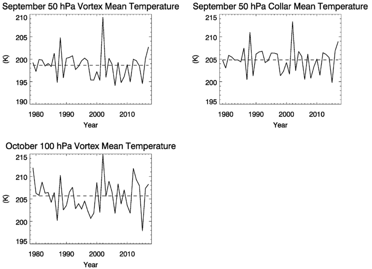
Figure 2 Mean temperature in the polar vortex at 50 hPa for September (upper left panel), for the vortex collar at 50 hPa in September (upper right panel) and polar vortex mean at 100 hPa in October (lower left panel). The dashed line represents the mean over the 1979-2017 period.
