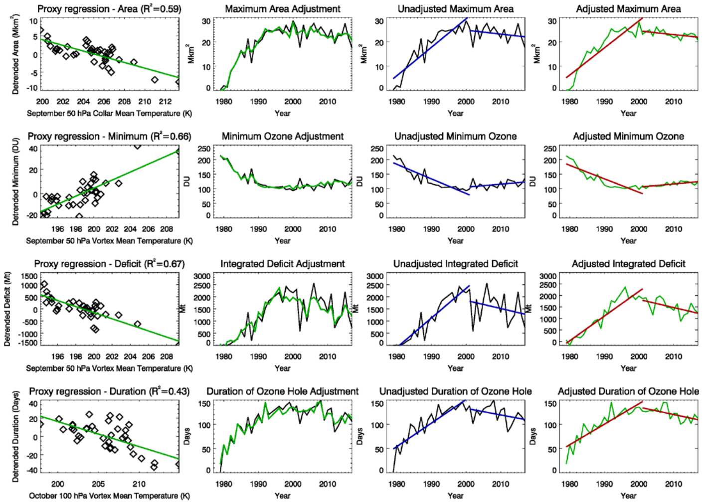
Figure 1 For each of the four metrics – Maximum 15-day averaged area of ozone hole, Minimum 15-day averaged total column ozone, Integrated ozone deficit and Duration of ozone hole - scatter plot of detrended metric versus selected temperature proxy and the linear fit (green); the adjusted (green) and unadjusted (black) proxy time-series; linear 1979-2001 and 2001-2017 trends (blue) of the unadjusted time series ; linear 1979-2001 and 2001-2017 trends (red) of the adjusted time series.
