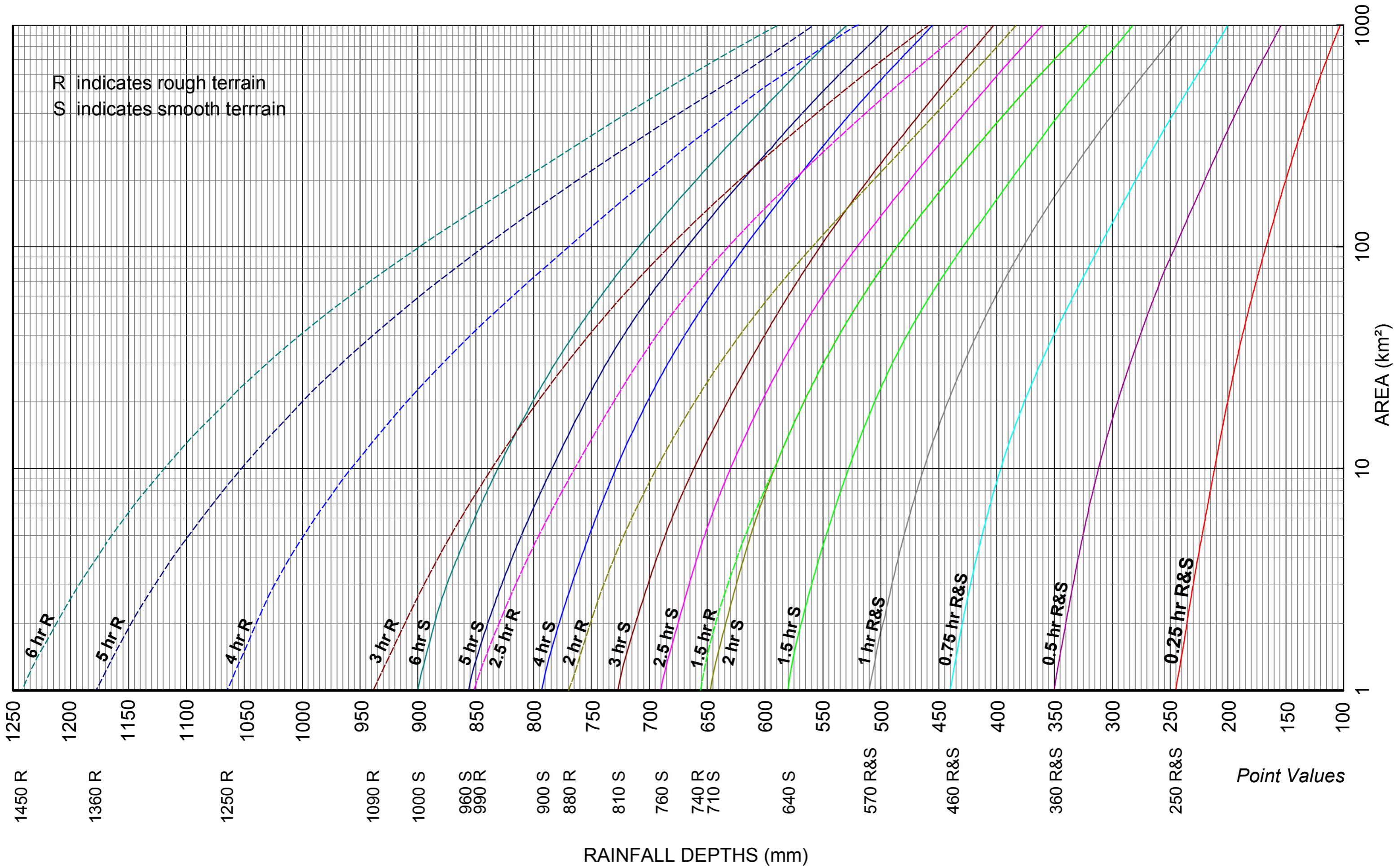
Depth-Duration-Area Curves of Short Duration Rainfall
