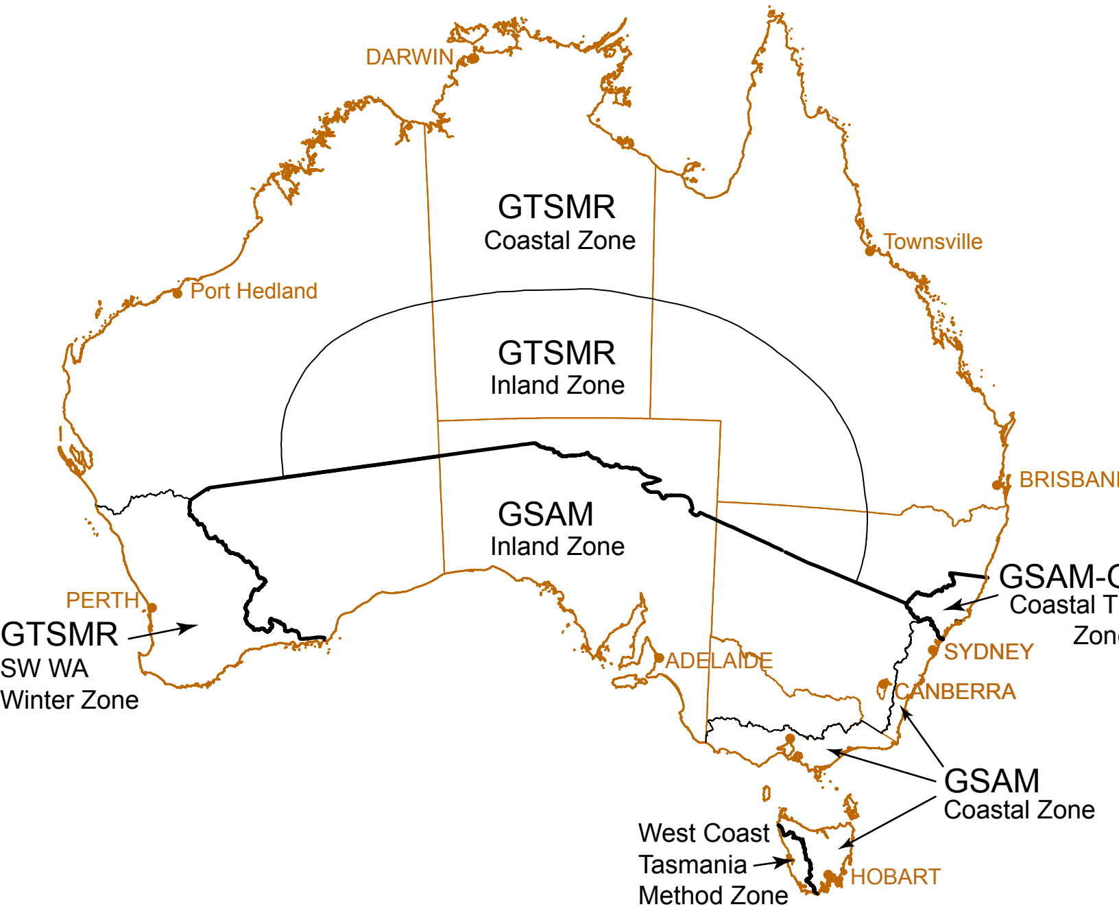
Figure 1 Generalised Tropical Storm - Revised Method and Generalised Southeast Australia Method zones.
