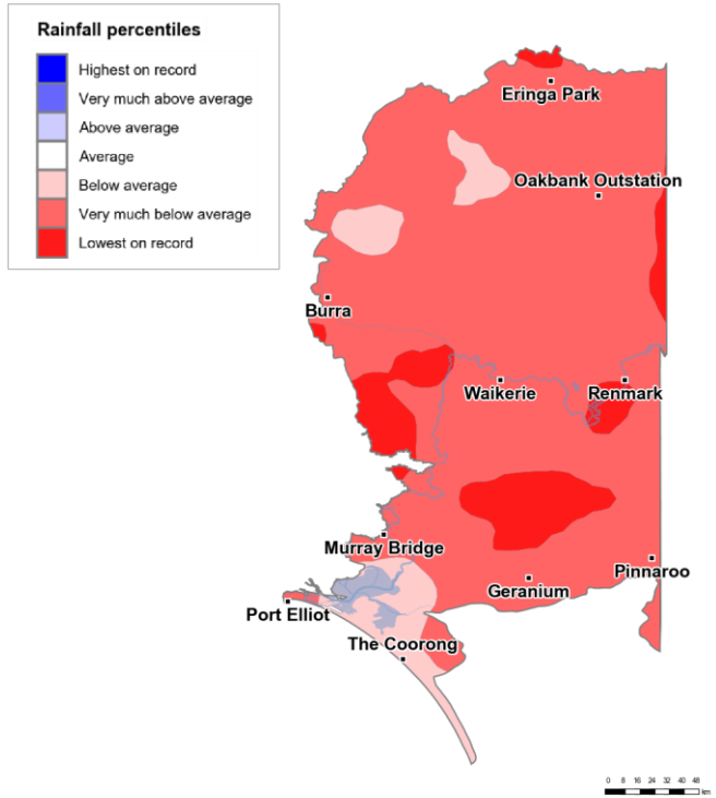
Figure 2: Rainfall percentiles since January 2017 (compared to 1900–2019 long-term average) (Jan 2017 to March 2021)
