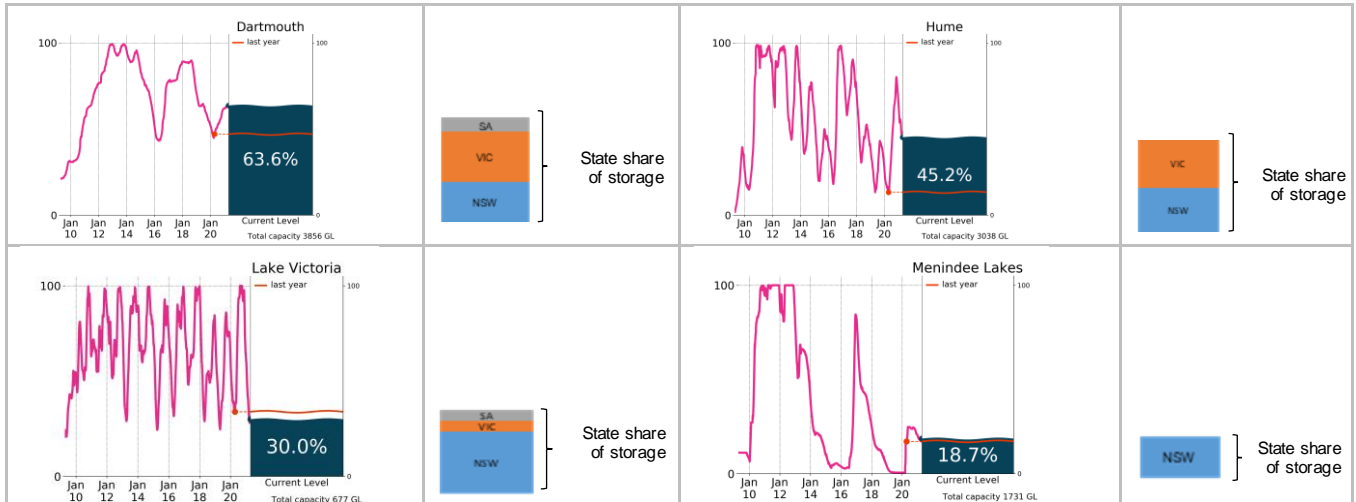
Figure 3: Current total storage (% of total capacity) as at 14 April 2021 compared to the last ten years (State shares updated end Mar 2021)
