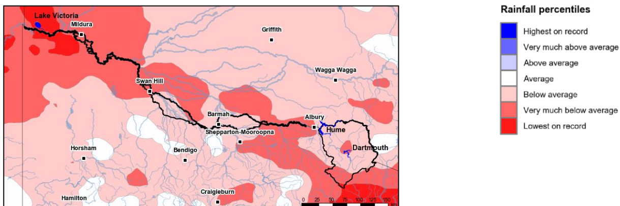
Figure 1: Rainfall totals for the last 30 days (17 March to 15 April 2021)
