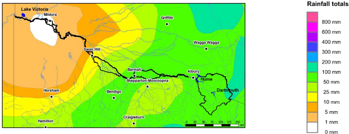
Figure 1: Rainfall totals for the last 30 days (17 March to 15 April 2021)
