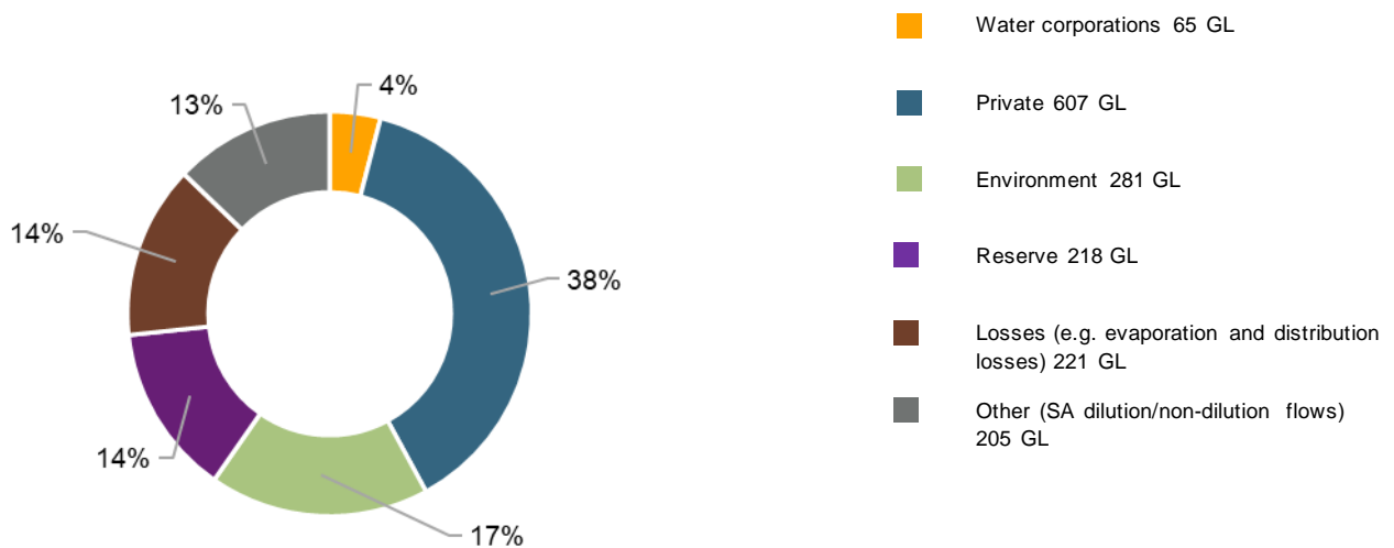
Figure 4: Volumes of water allocations currently available/remaining (% of total remaining) (as at 1 April 2021)
