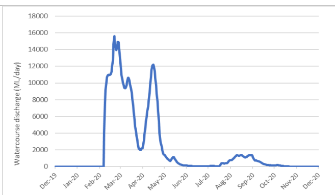
Figure 3: Watercourse discharge (ML per day) for last 12 months at selected gauges in the Barwon–Darling Watercourse (as at 15 December 2020)
