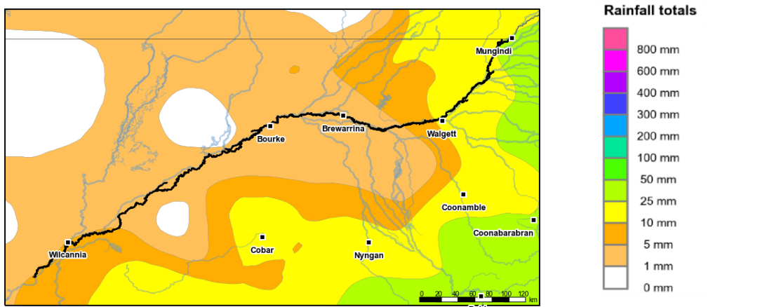
Figure 1: Rainfall totals for the last 30 days (16 Nov to 15 Dec 2020)
