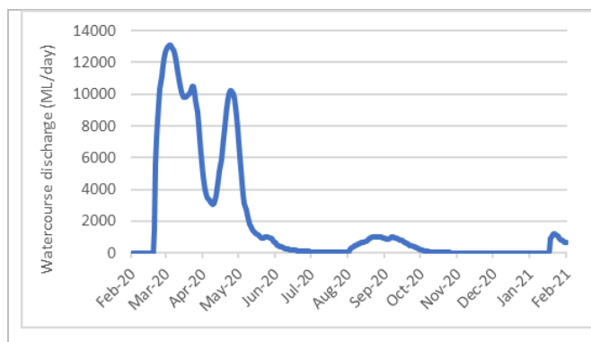
Figure 3: Watercourse discharge (ML per day) for last 12 months at selected gauges in the Barwon–Darling Watercourse (as at 15 February 2021)
