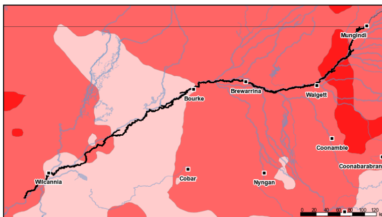
Figure 1: Rainfall totals for the last 30 days (17 Jan to 15 Feb 2021)
