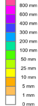
Rainfall totals
