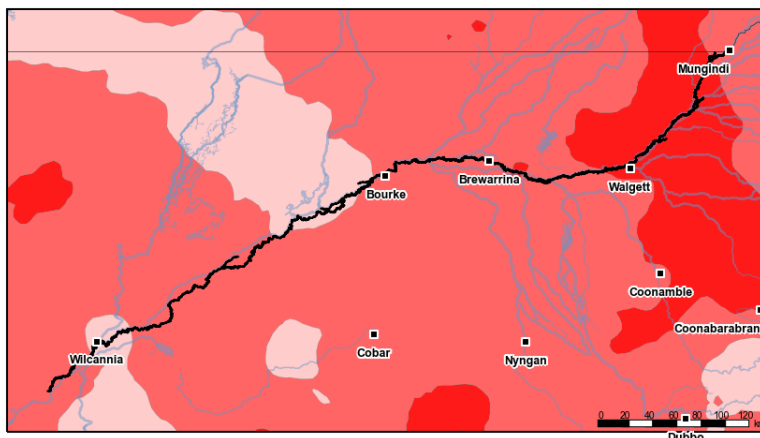
Figure 2: Rainfall percentiles since January 2017 (compared to 1900–2019 long-term average) (Jan 2017 to Oct 2020)
