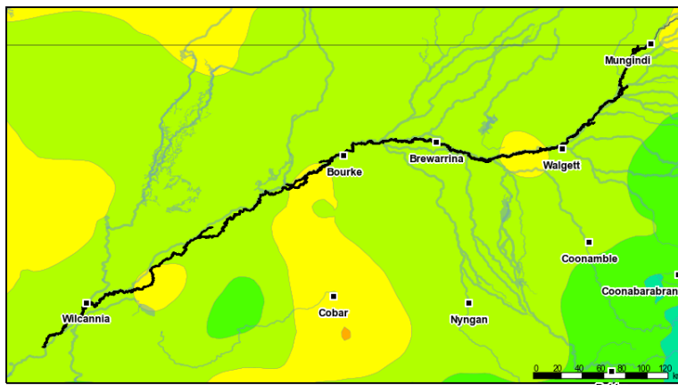
Figure 1: Rainfall totals for the last 30 days (18 Oct to 16 Nov 2020)
