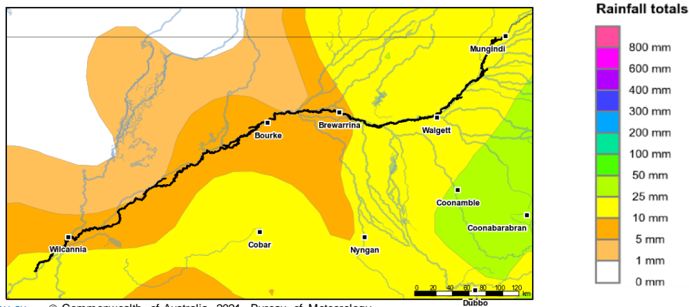
Figure 1: Rainfall totals for the last 30 days (18 April to 17 May 2021)
