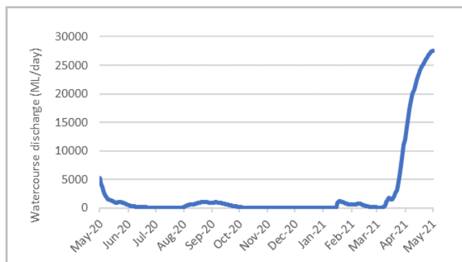
Figure 3: Watercourse discharge (ML per day) for last 12 months at selected gauges in the Barwon–Darling Watercourse (as at 17 May 2021)
