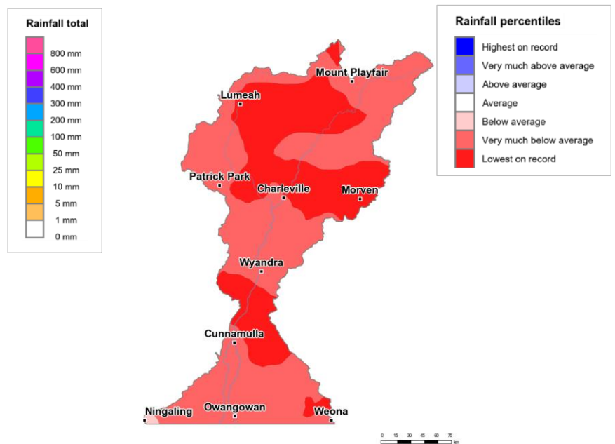
Figure 2: Rainfall percentiles since January 2017 (compared to 1900–2019 long-term average) (Jan 2017 to Nov 2020)
