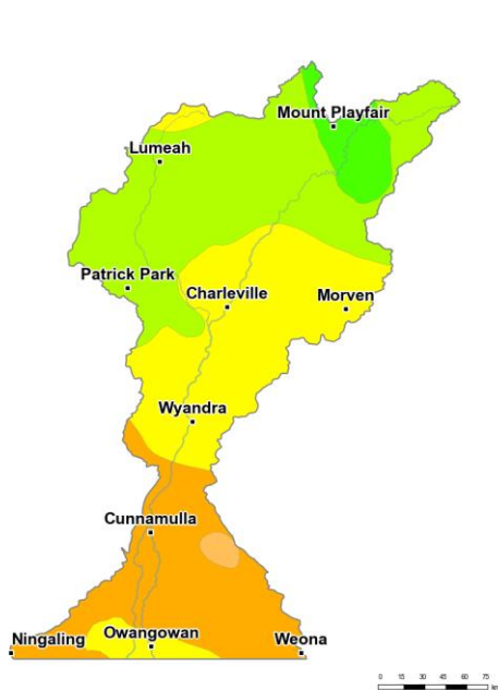
Figure 1: Rainfall totals for the last 30 days (2 Nov to 1 Dec 2020)
