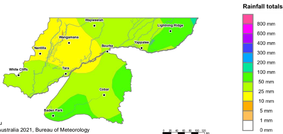
Figure 1: Rainfall totals for the last 30 days (3 Jan to 1 Feb 2021)
