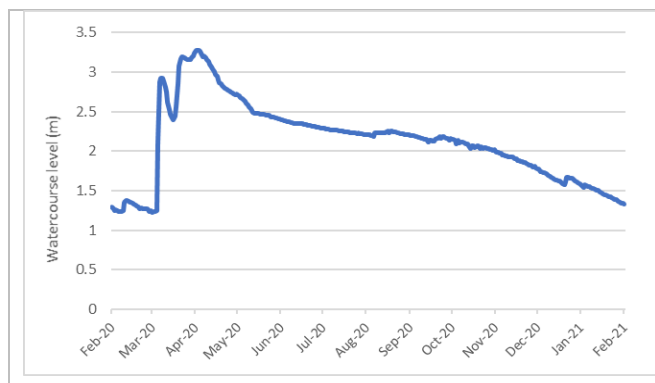
Figure 3: Water course levels for last 12 months at selected gauges in the Intersecting Streams catchment (as at 1 February 2021)
