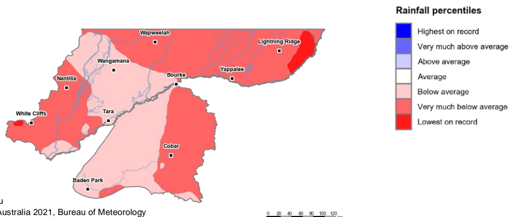
Figure 2: Rainfall percentiles since January 2017 (compared to 1900–2019 long-term average) (Jan 2017 to Jan 2021)
